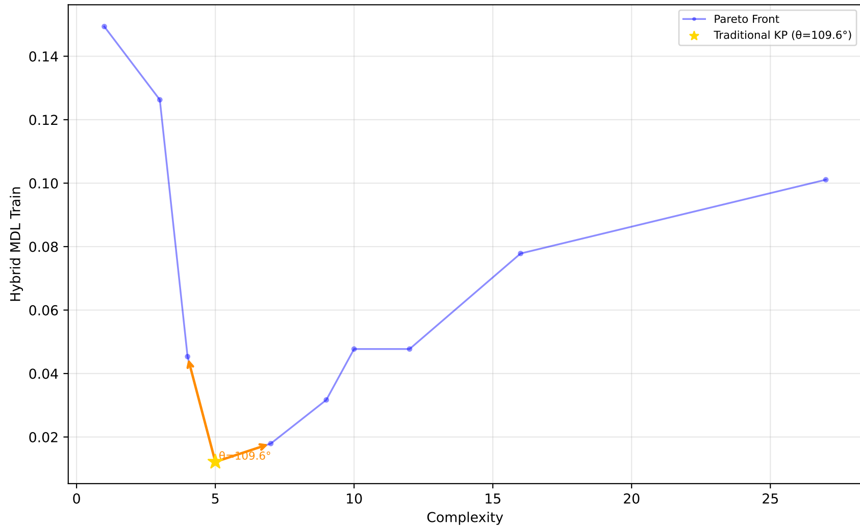
523_analcatdata_neavote - Run 17 - SVP - Hybrid MDL Train \lambda_1=0.00 , \lambda_2=0.20 , \lambda_3=0.00 | Difficulty: 1.00 | Method: hmr
