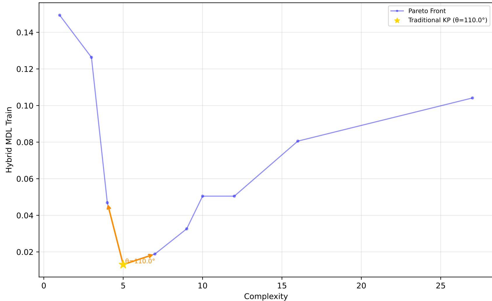
523_analcatdata_neavote - Run 17 - SVP - Hybrid MDL Train \lambda_1=0.00, \lambda_2=0.90, \lambda_3=0.00 | Difficulty: 1.00 | Method: hmr
