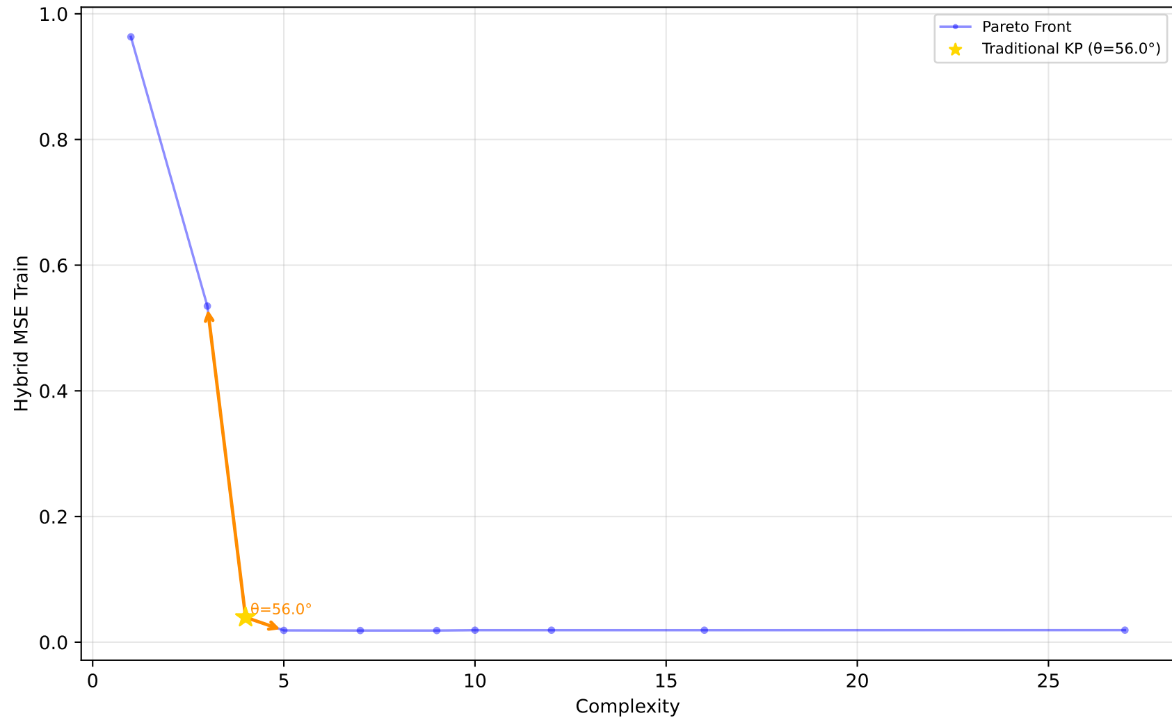
523_analcatdata_neavote - Run 17 - SVP - Hybrid MSE Train \lambda_1=0.00 , \lambda_2=0.20 , \lambda_3=0.00 | Difficulty: 1.00 | Method: hmr
