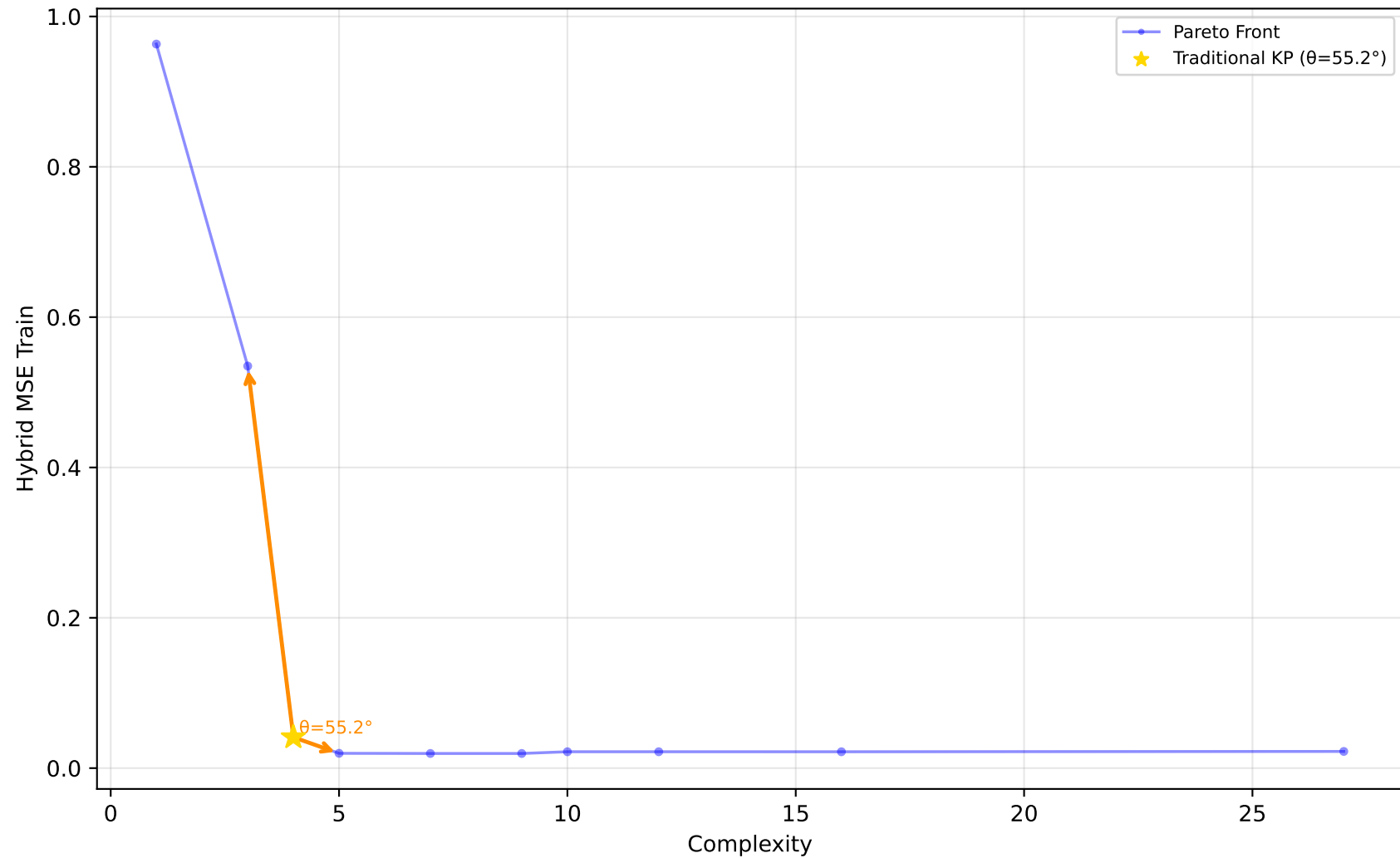
523_analcatdata_neavote - Run 17 - SVP - Hybrid MSE Train \lambda_1=0.00, \lambda_2=0.90, \lambda_3=0.00 | Difficulty: 1.00 | Method: hmr
