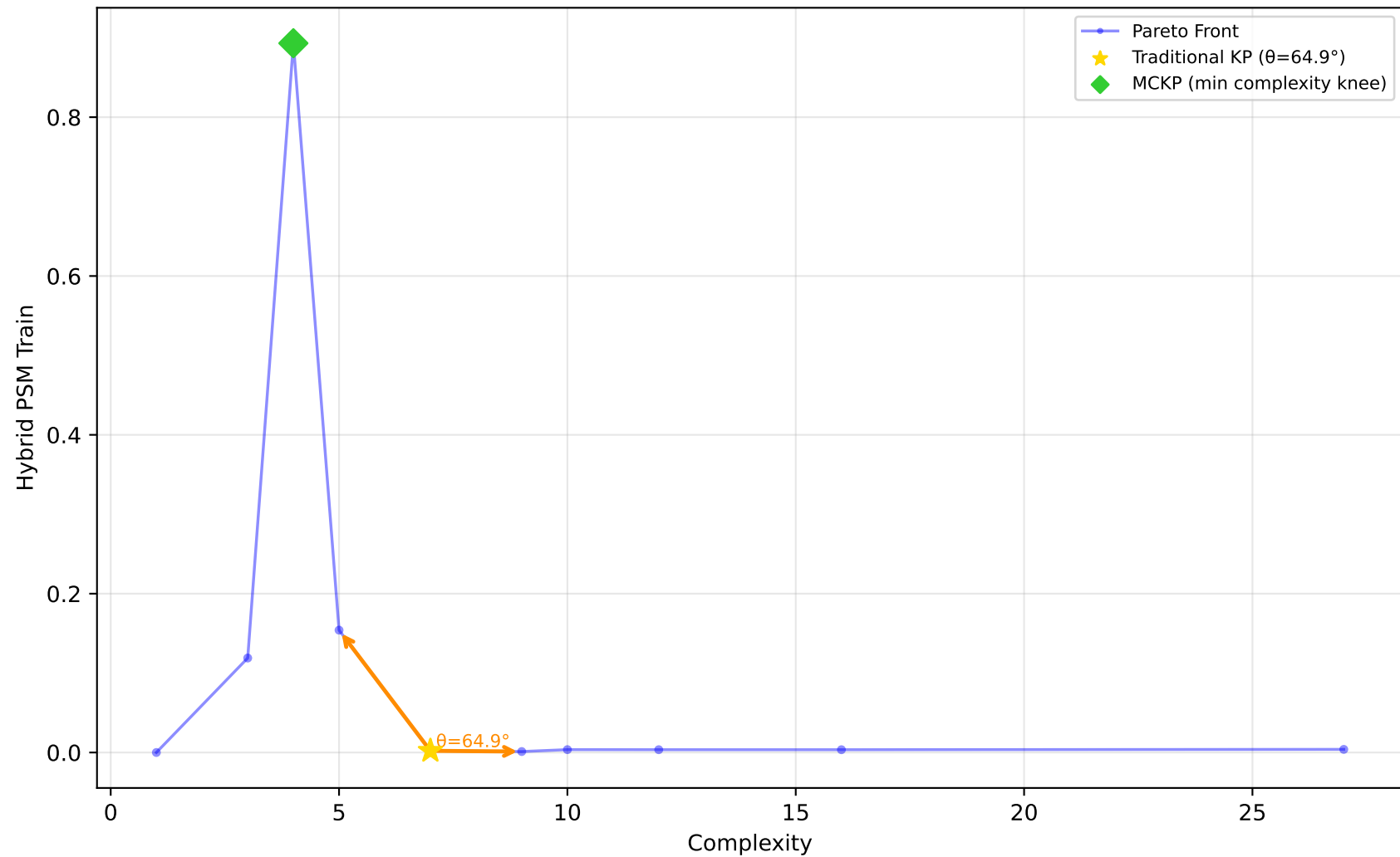
523_analcatdata_neavote - Run 17 - SVP - Hybrid PSM Train \lambda_1=0.00, \lambda_2=0.90, \lambda_3=0.00 | Difficulty: 1.00 | Method: hmr
