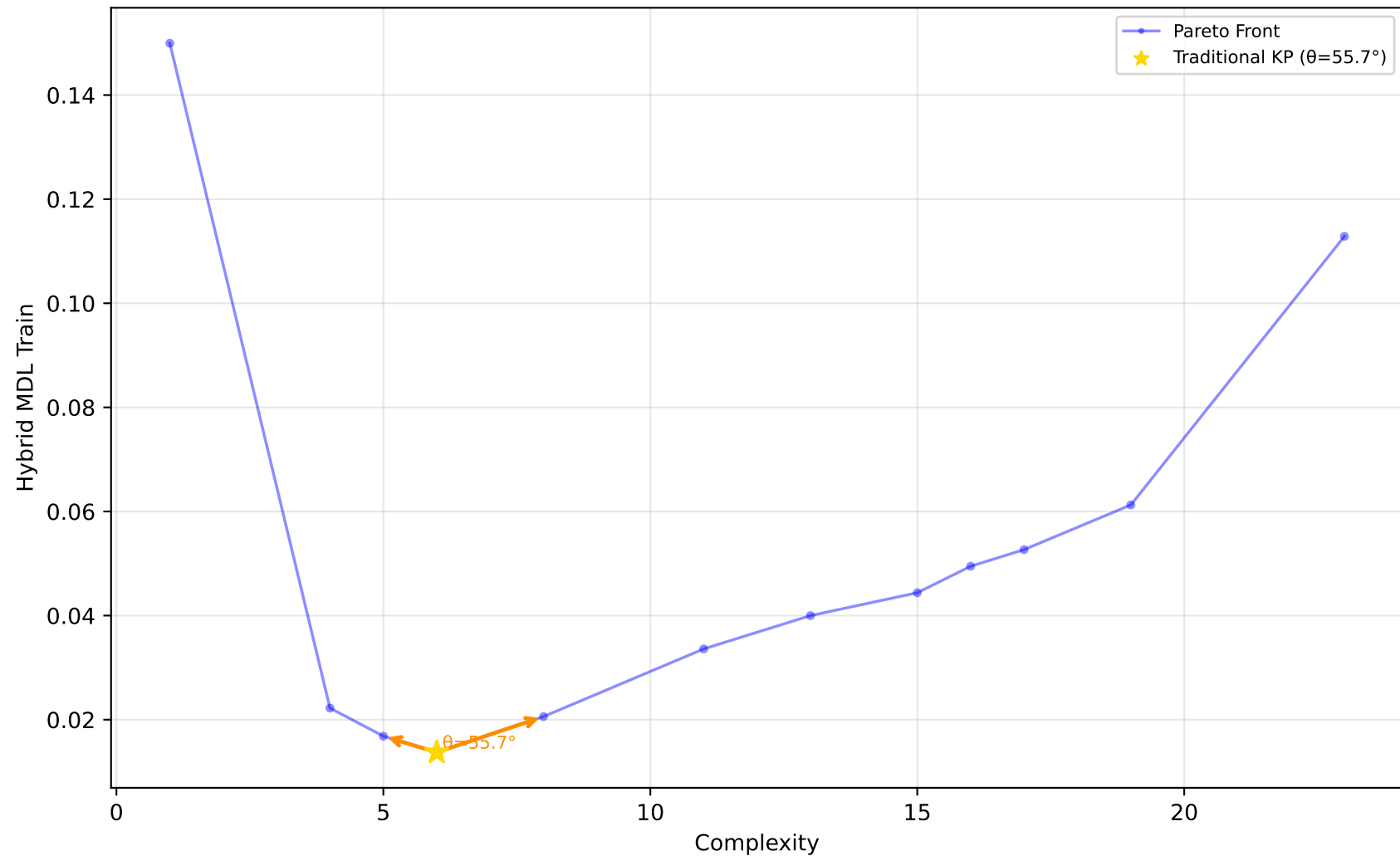
523_analcatdata_neavote - Run 18 - MVP - Hybrid MDL Train \lambda_1=0.00, \lambda_2=0.10, \lambda_3=0.00 | Difficulty: 1.00 | Method: hmr
