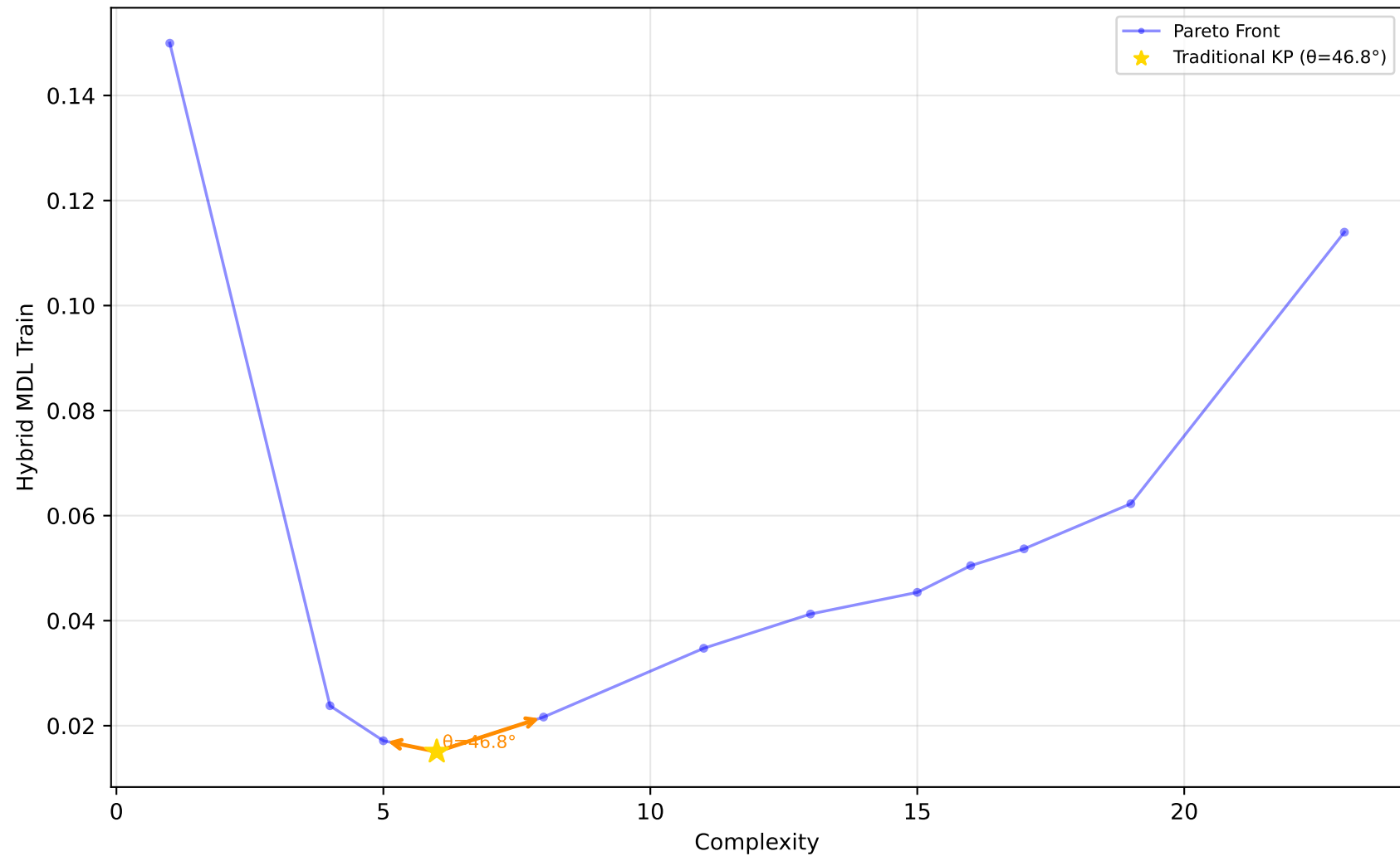
523_analcatdata_neavote - Run 18 - MVP - Hybrid MDL Train \lambda_1=0.00, \lambda_2=0.40, \lambda_3=0.00 | Difficulty: 1.00 | Method: hmr
