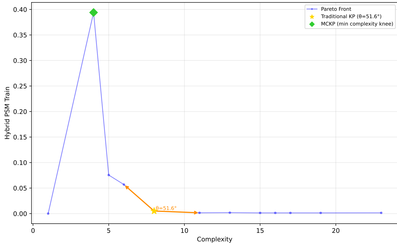
523_analcatdata_neavote - Run 18 - MVP - Hybrid PSM Train \lambda_1=0.00 , \lambda_2=0.40 , \lambda_3=0.00 | Difficulty: 1.00 | Method: hmr
