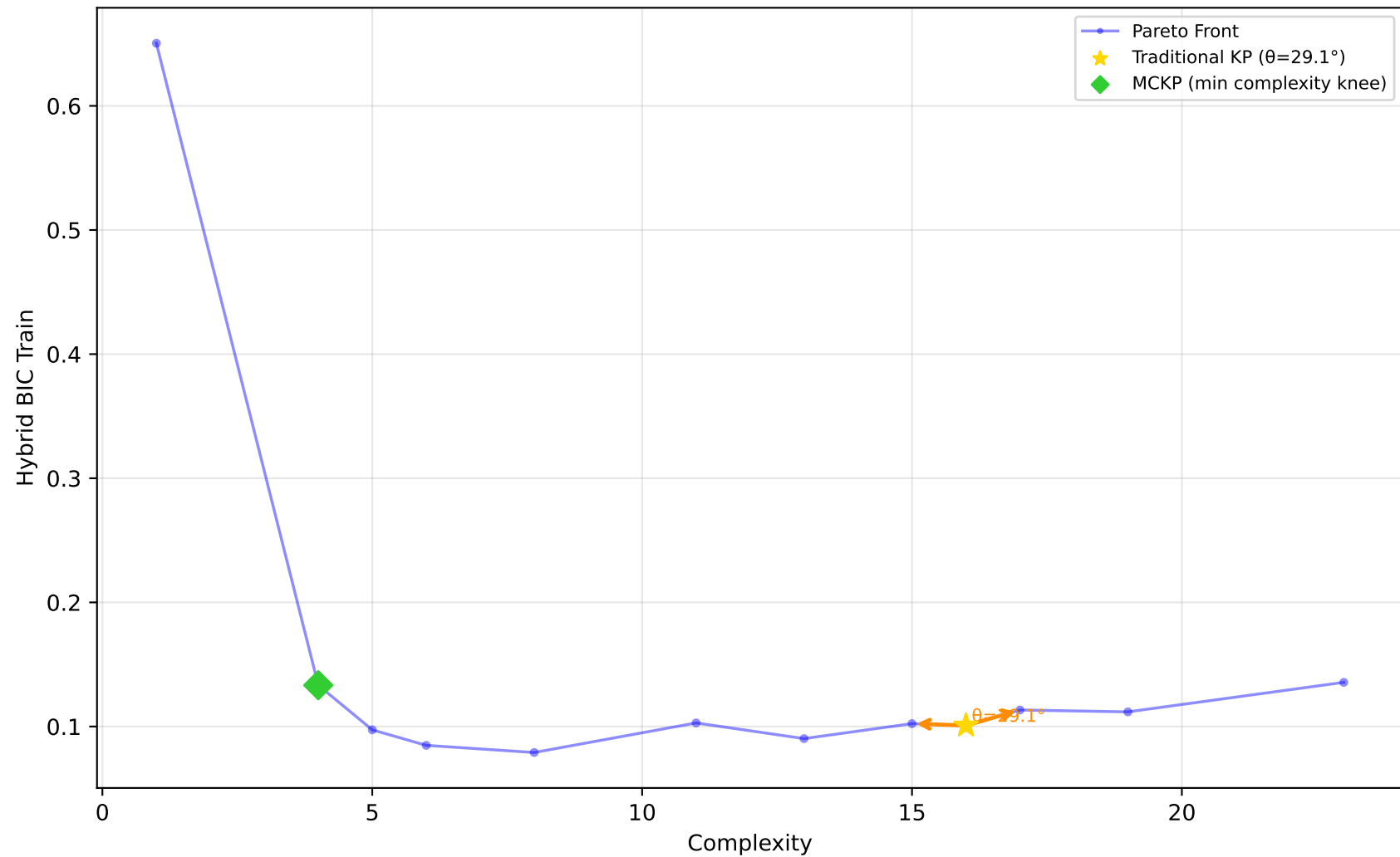
523_analcatdata_neavote - Run 18 - SVP - Hybrid BIC Train \lambda_1=0.00 , \lambda_2=0.90 , \lambda_3=0.00 | Difficulty: 1.00 | Method: hmr
