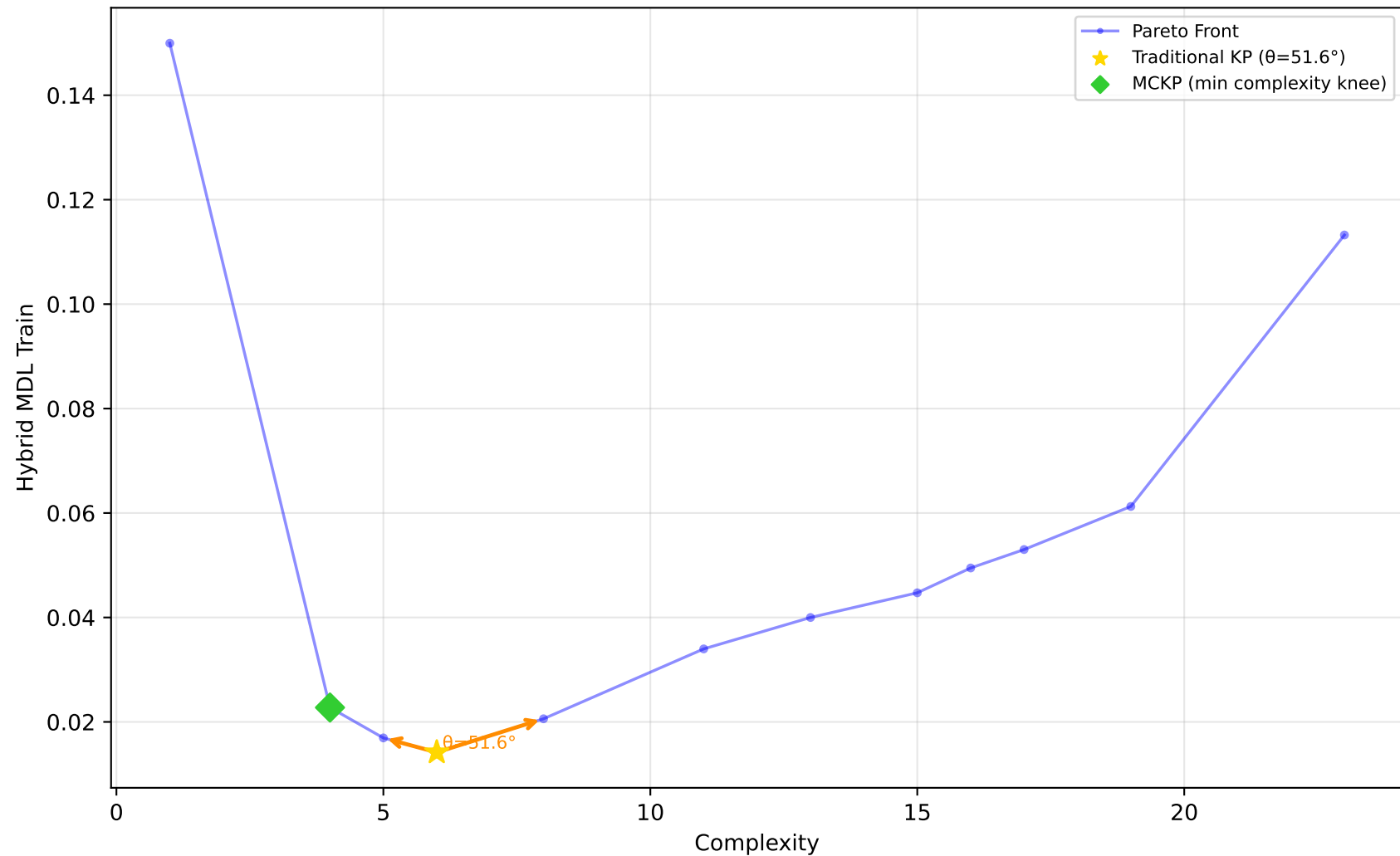
523_analcatdata_neavote - Run 18 - SVP - Hybrid MDL Train \lambda_1=0.00 , \lambda_2=0.20 , \lambda_3=0.00 | Difficulty: 1.00 | Method: hmr
