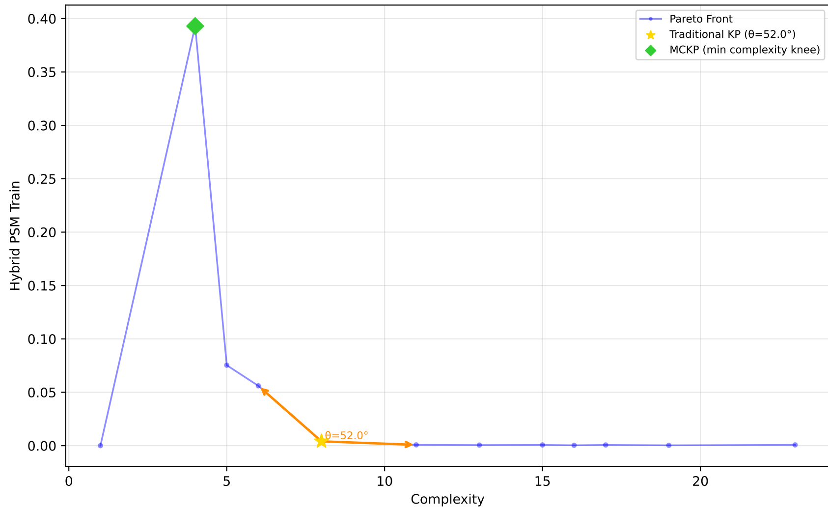
523_analcatdata_neavote - Run 18 - SVP - Hybrid PSM Train \lambda_1=0.00 , \lambda_2=0.20 , \lambda_3=0.00 | Difficulty: 1.00 | Method: hmr
