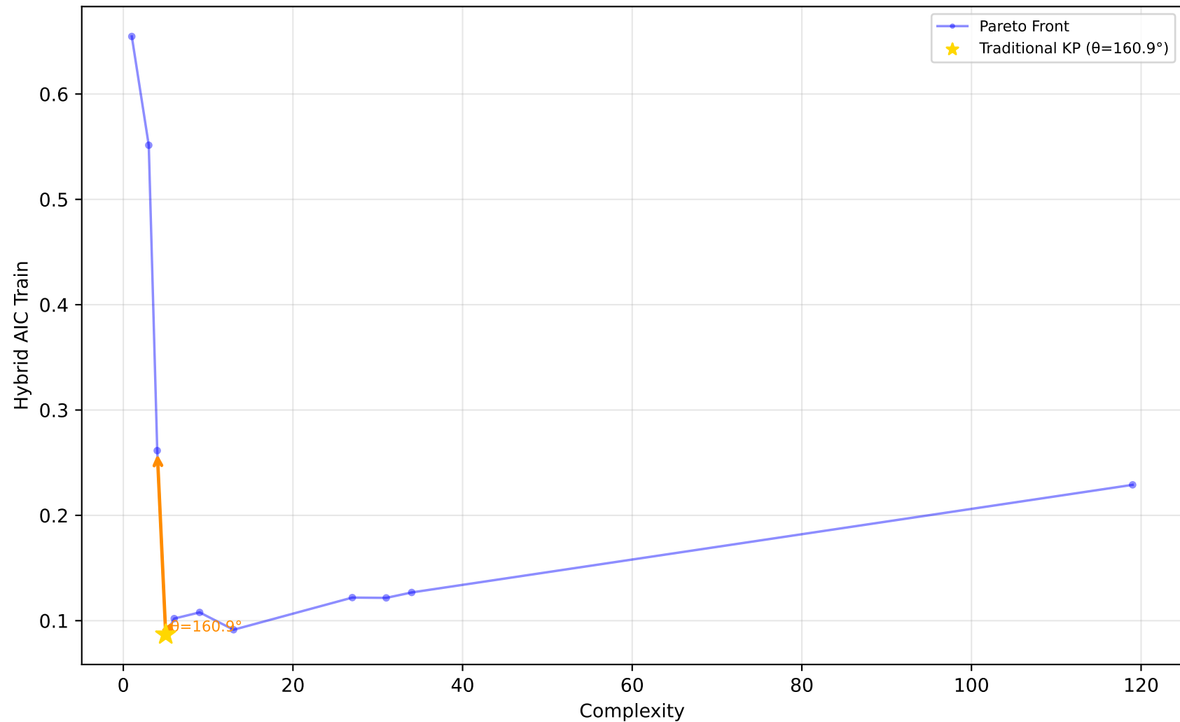
523_analcatdata_neavote - Run 19 - SVP - Hybrid AIC Train \lambda_1=0.00, \lambda_2=0.90, \lambda_3=0.00 | Difficulty: 1.00 | Method: hmr
