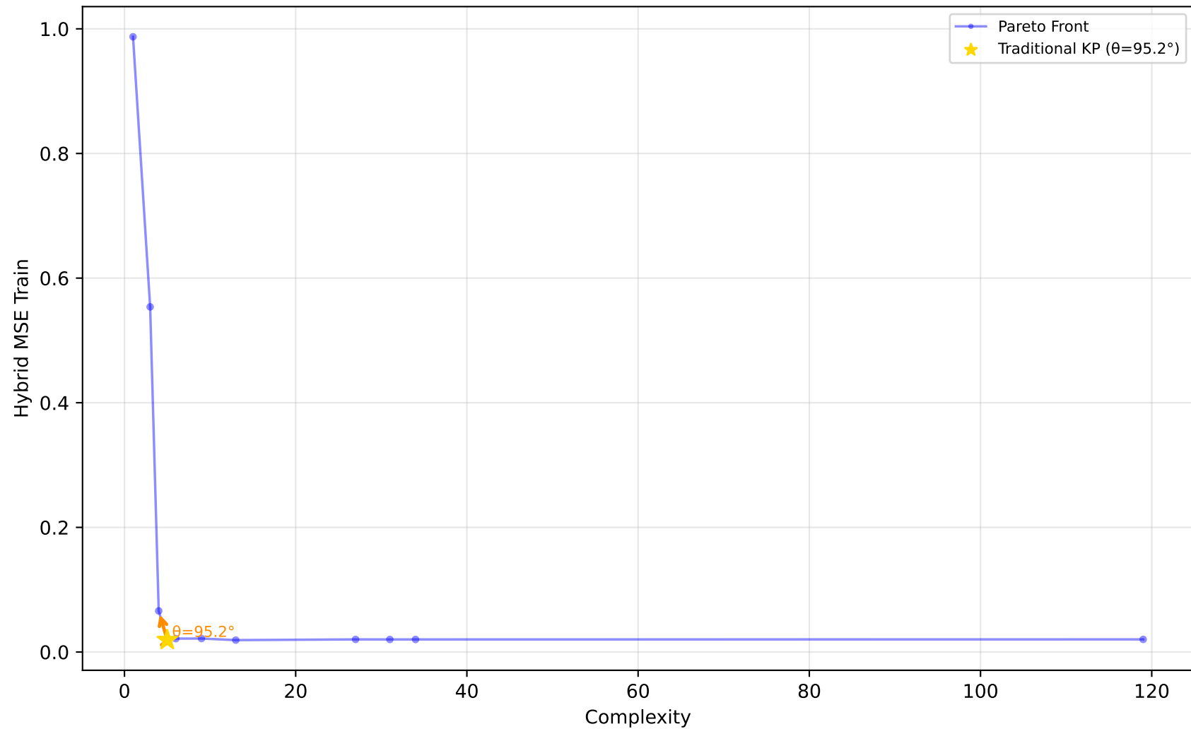
523_analcatdata_neavote - Run 19 - SVP - Hybrid MSE Train \lambda_1=0.00, \lambda_2=0.20, \lambda_3=0.00 | Difficulty: 1.00 | Method: hmr
