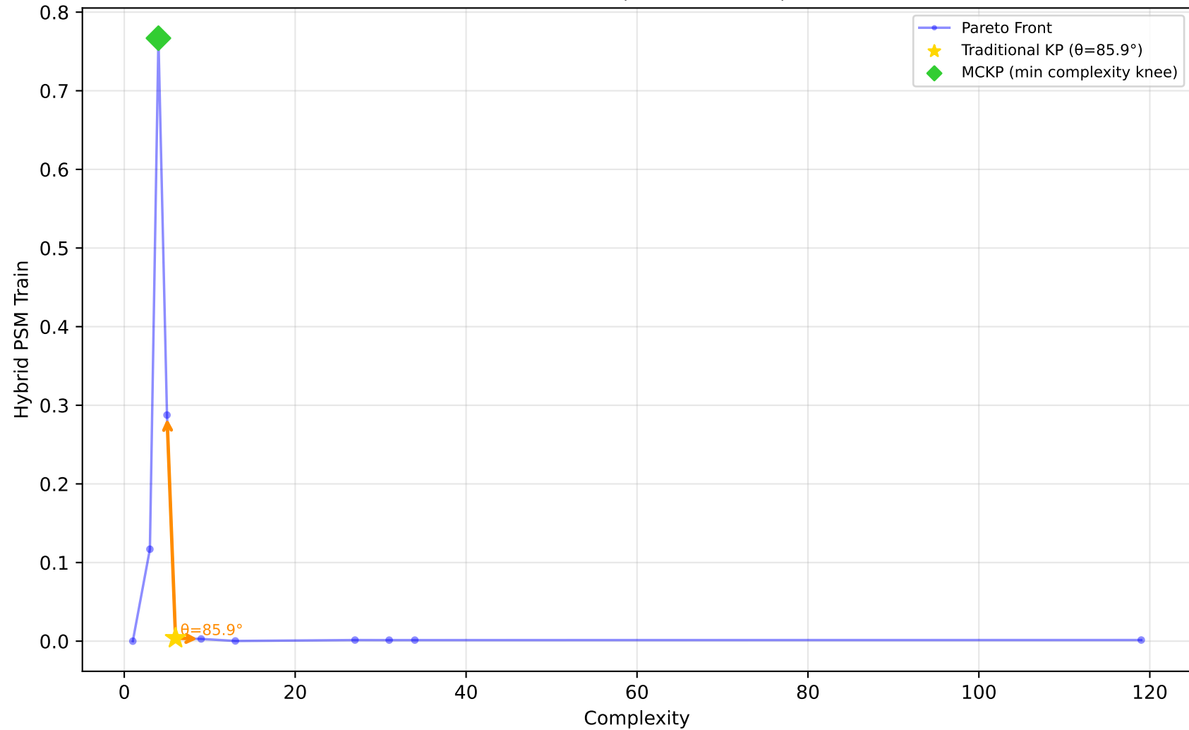
523_analcatdata_neavote - Run 19 - SVP - Hybrid PSM Train \lambda_1=0.00, \lambda_2=0.20, \lambda_3=0.00 | Difficulty: 1.00 | Method: hmr
