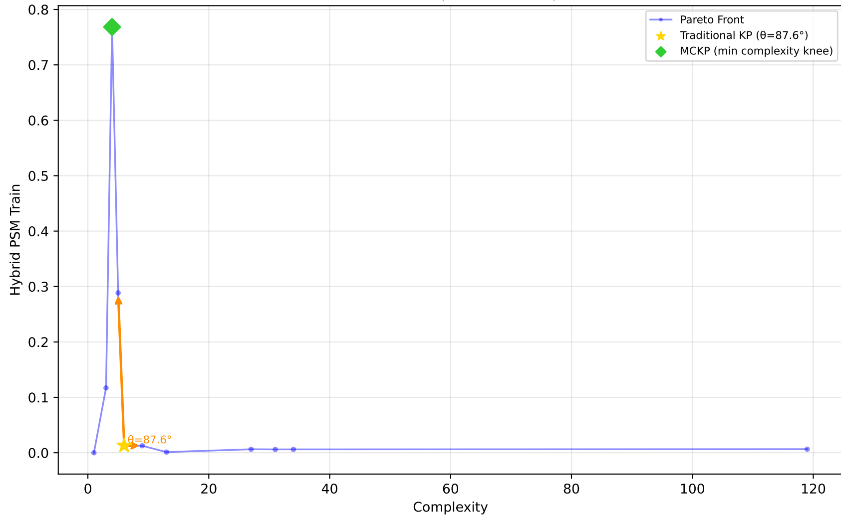
523_analcatdata_neavote - Run 19 - SVP - Hybrid PSM Train \lambda_1=0.00, \lambda_2=0.90, \lambda_3=0.00 | Difficulty: 1.00 | Method: hmr
