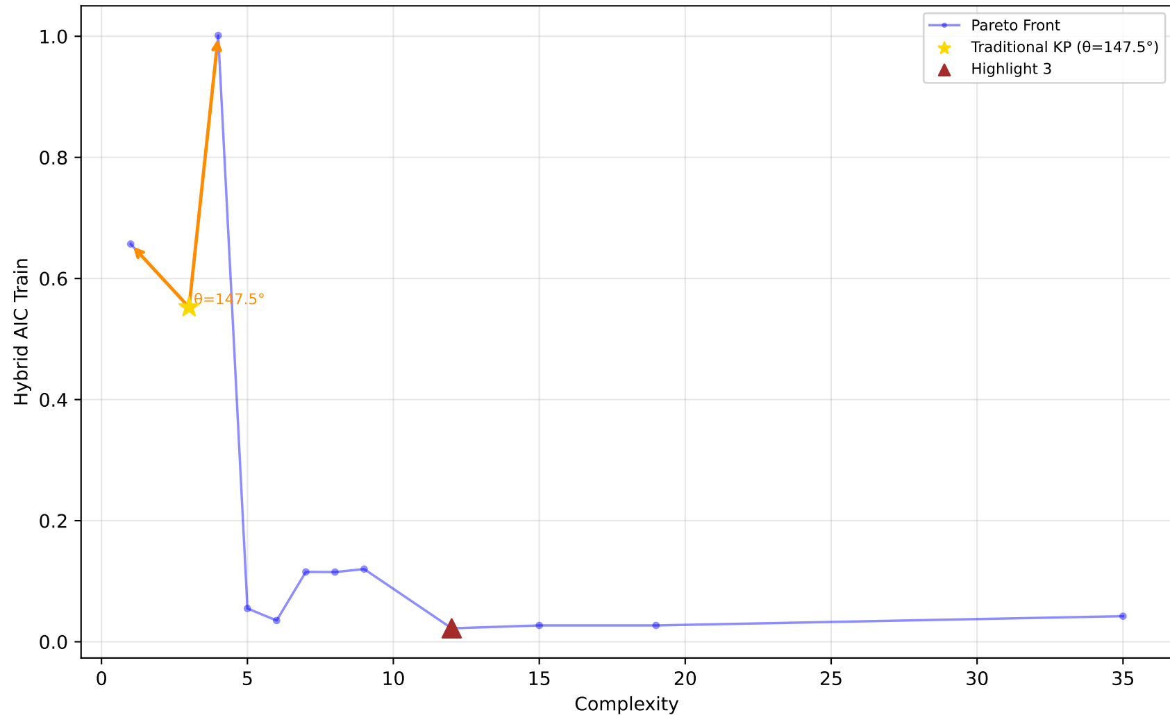
523_analcatdata_neavote - Run 1 - MVP - Hybrid AIC Train \lambda_1=0.00, \lambda_2=0.10, \lambda_3=0.00 | Difficulty: 1.00 | Method: hmr
