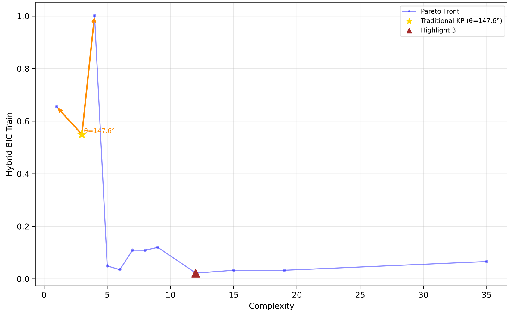
523_analcatdata_neavote - Run 1 - MVP - Hybrid BIC Train \lambda_1=0.00, \lambda_2=0.10, \lambda_3=0.00 | Difficulty: 1.00 | Method: hmr
