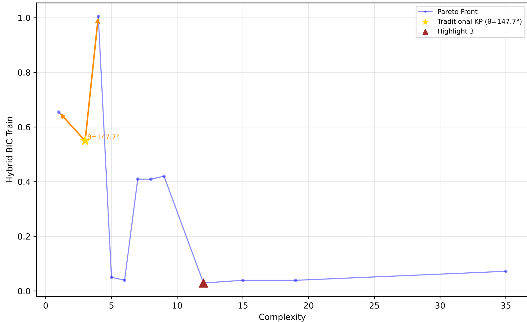
523_analcatdata_neavote - Run 1 - MVP - Hybrid BIC Train \lambda_1=0.00, \lambda_2=0.40, \lambda_3=0.00 | Difficulty: 1.00 | Method: hmr
