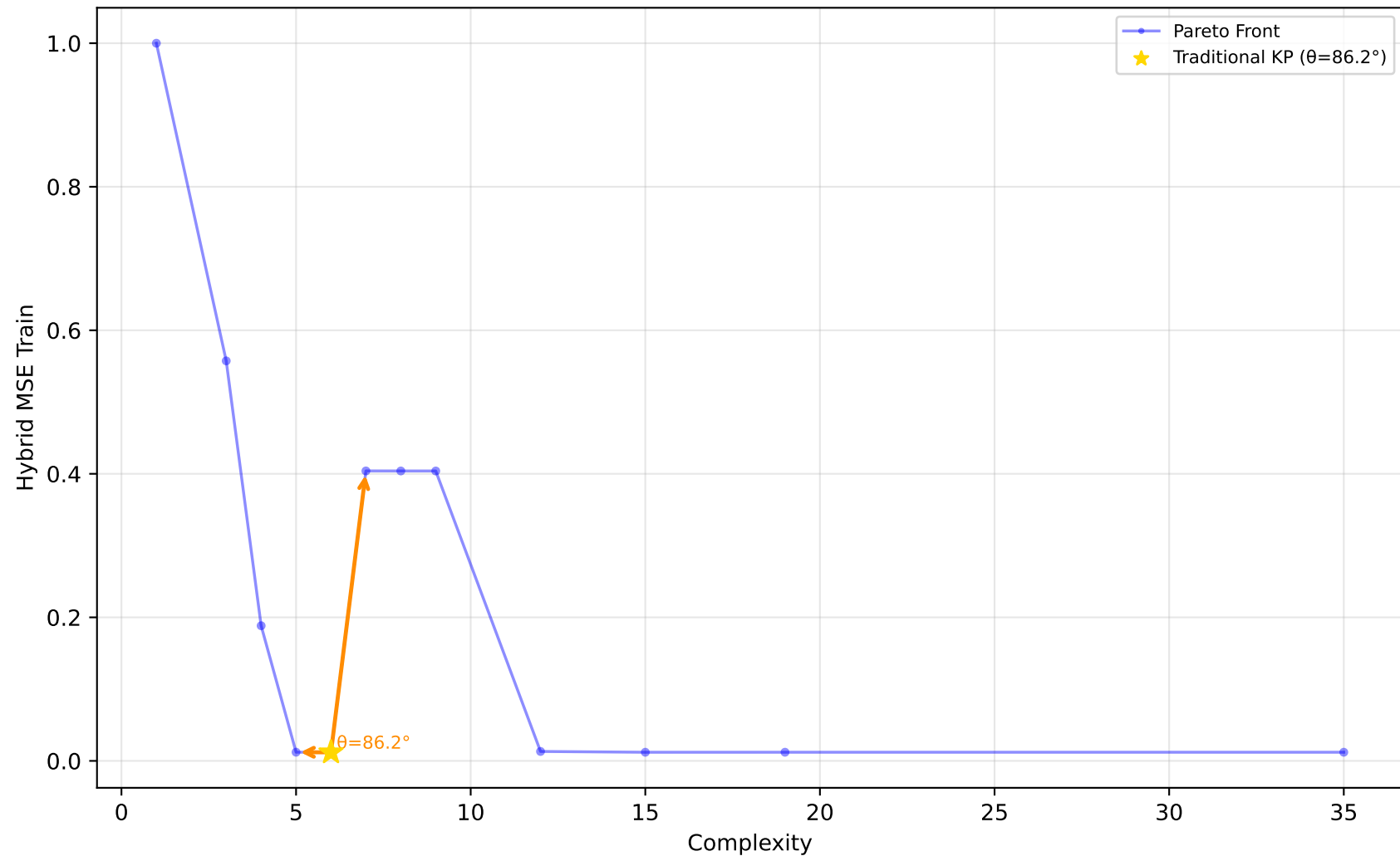
523_analcatdata_neavote - Run 1 - MVP - Hybrid MSE Train \lambda_1=0.00, \lambda_2=0.40, \lambda_3=0.00 | Difficulty: 1.00 | Method: hmr
