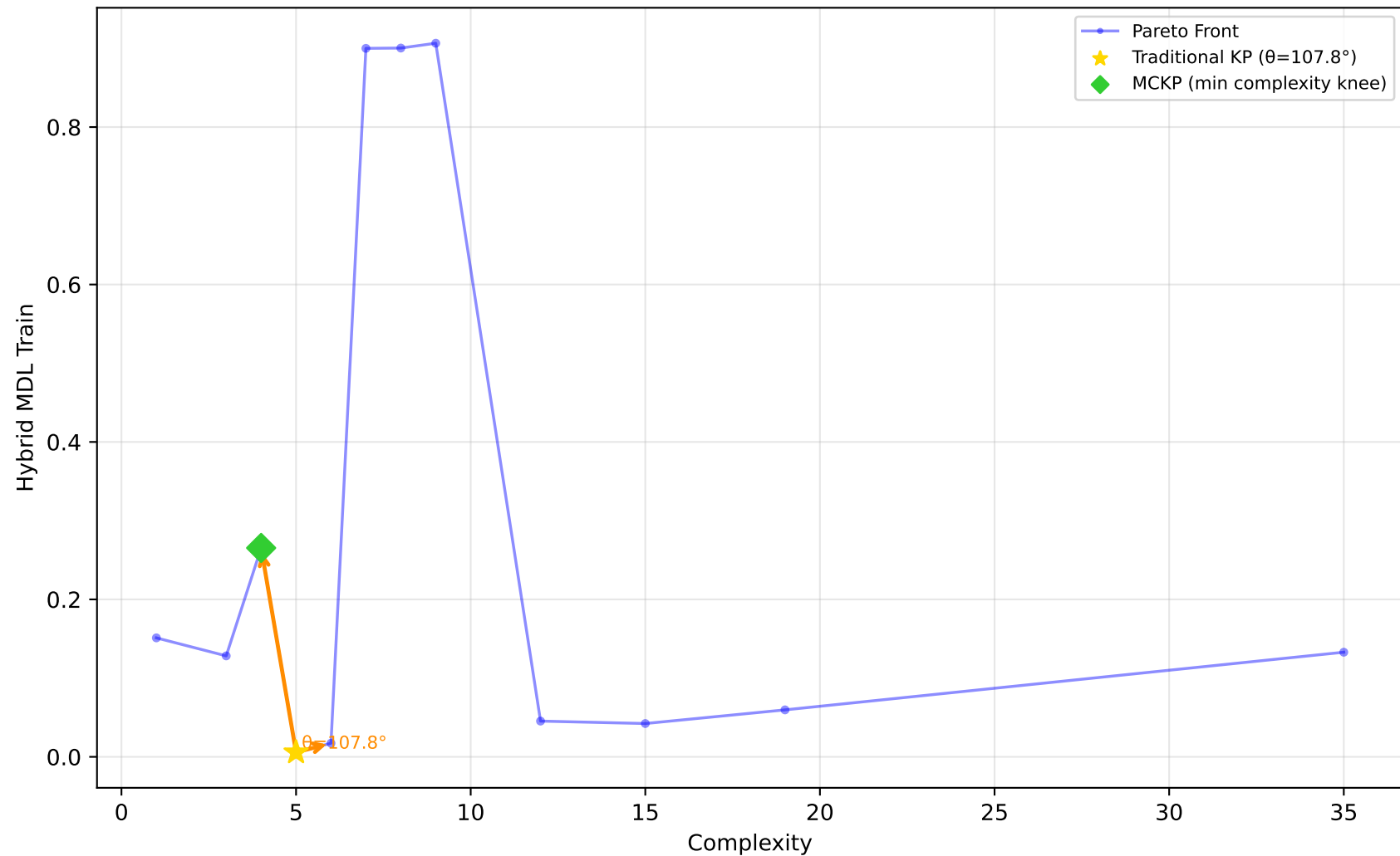
523_analcatdata_neavote - Run 1 - SVP - Hybrid MDL Train \lambda_1=0.00, \lambda_2=0.90, \lambda_3=0.00 | Difficulty: 1.00 | Method: hmr
