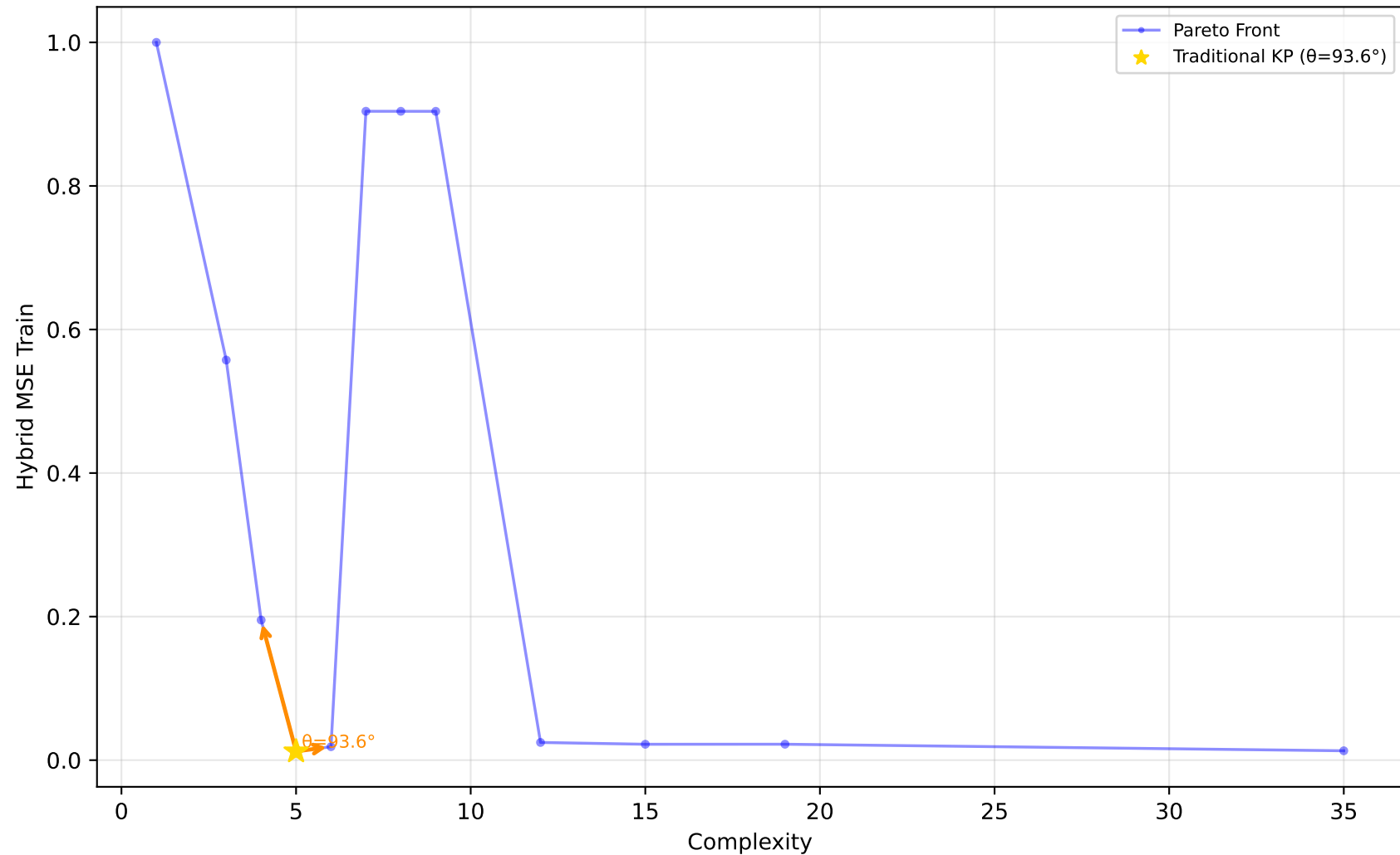
523_analcatdata_neavote - Run 1 - SVP - Hybrid MSE Train \lambda_1=0.00, \lambda_2=0.90, \lambda_3=0.00 | Difficulty: 1.00 | Method: hmr
