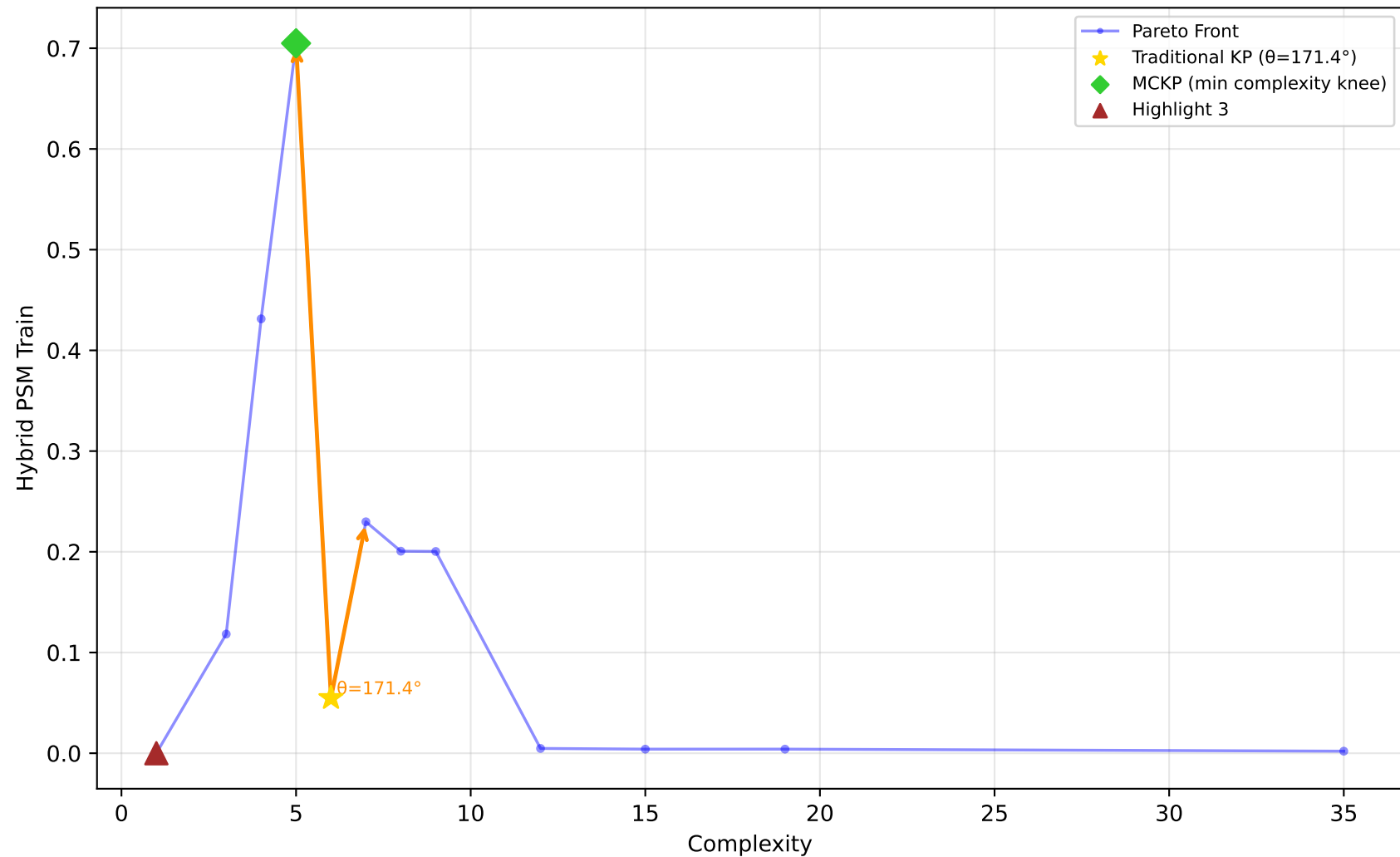
523_analcatdata_neavote - Run 1 - SVP - Hybrid PSM Train \lambda_1=0.00, \lambda_2=0.20, \lambda_3=0.00 | Difficulty: 1.00 | Method: hmr
