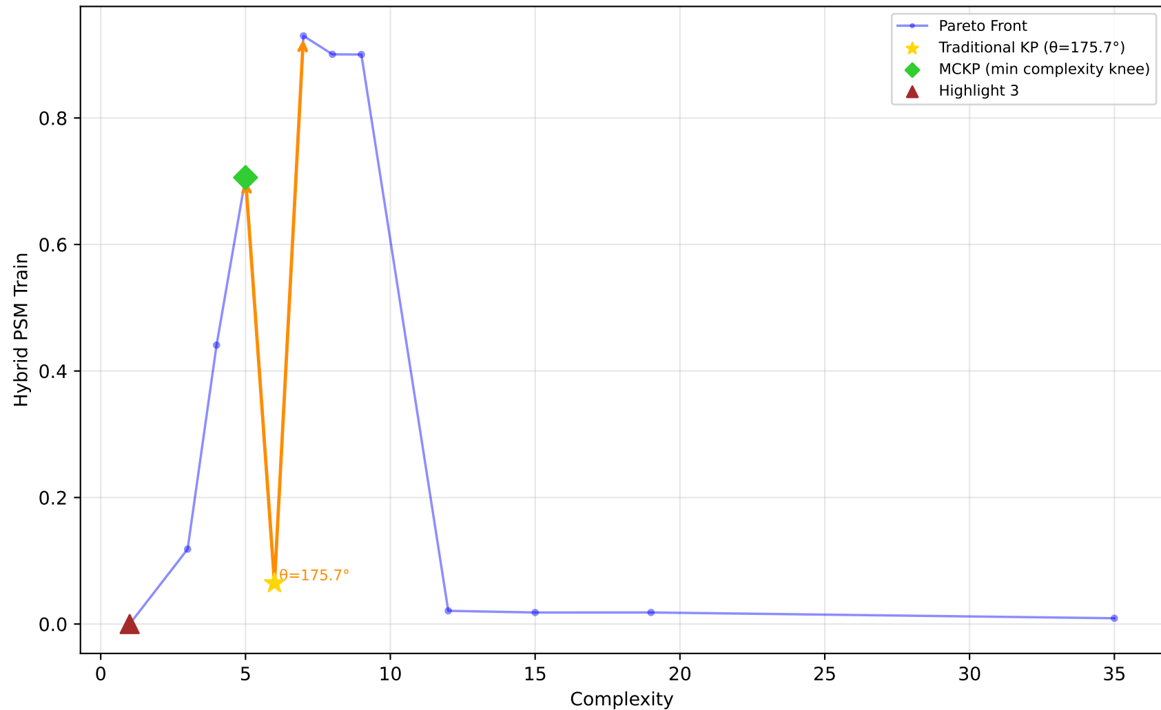
523_analcatdata_neavote - Run 1 - SVP - Hybrid PSM Train \lambda_1=0.00, \lambda_2=0.90, \lambda_3=0.00 | Difficulty: 1.00 | Method: hmr
