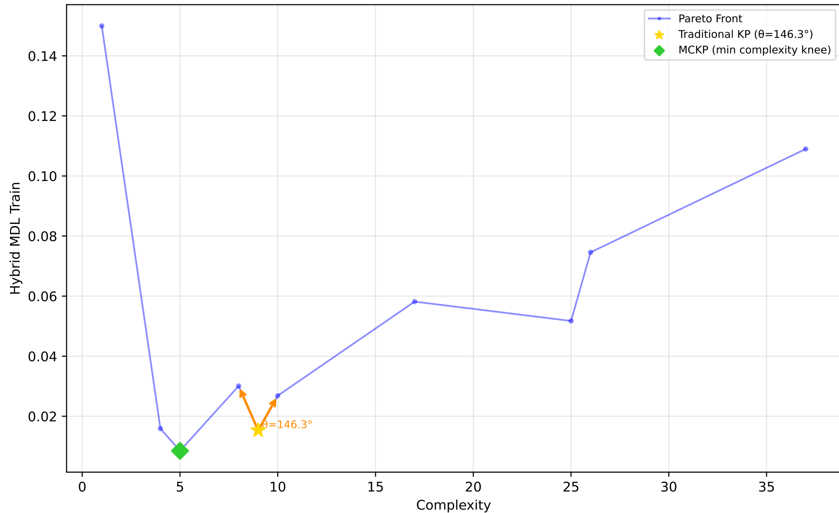
523_analcatdata_neavote - Run 20 - MVP - Hybrid MDL Train \lambda_1=0.00, \lambda_2=0.10, \lambda_3=0.00 | Difficulty: 1.00 | Method: hmr
