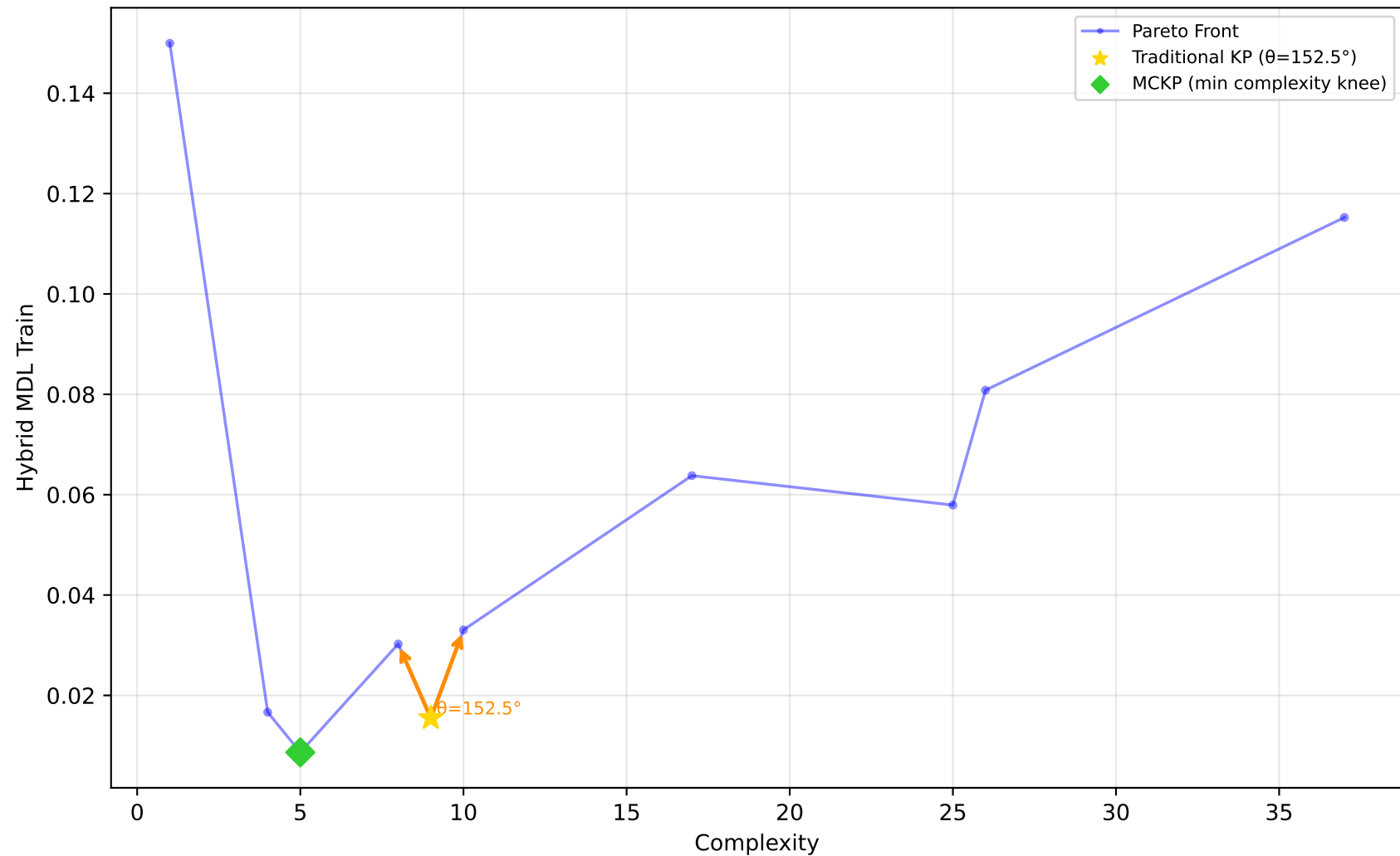
523_analcatdata_neavote - Run 20 - MVP - Hybrid MDL Train \lambda_1=0.00 , \lambda_2=0.40 , \lambda_3=0.00 | Difficulty: 1.00 | Method: hmr
