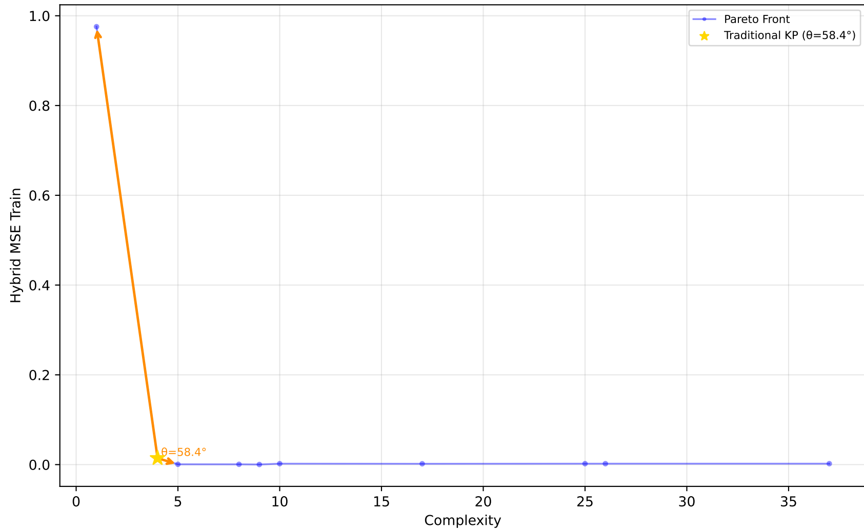
523_analcatdata_neavote - Run 20 - MVP - Hybrid MSE Train \lambda_1=0.00, \lambda_2=0.10, \lambda_3=0.00 | Difficulty: 1.00 | Method: hmr
