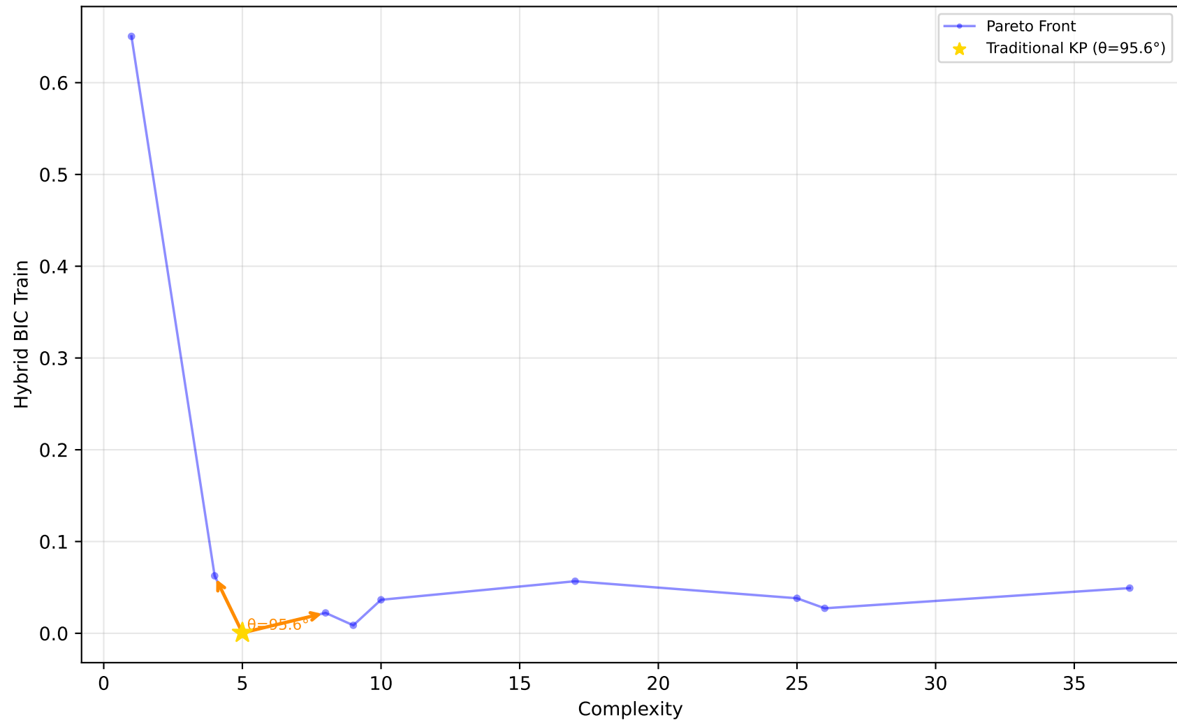
523_analcatdata_neavote - Run 20 - SVP - Hybrid BIC Train \lambda_1=0.00, \lambda_2=0.90, \lambda_3=0.00 | Difficulty: 1.00 | Method: hmr
