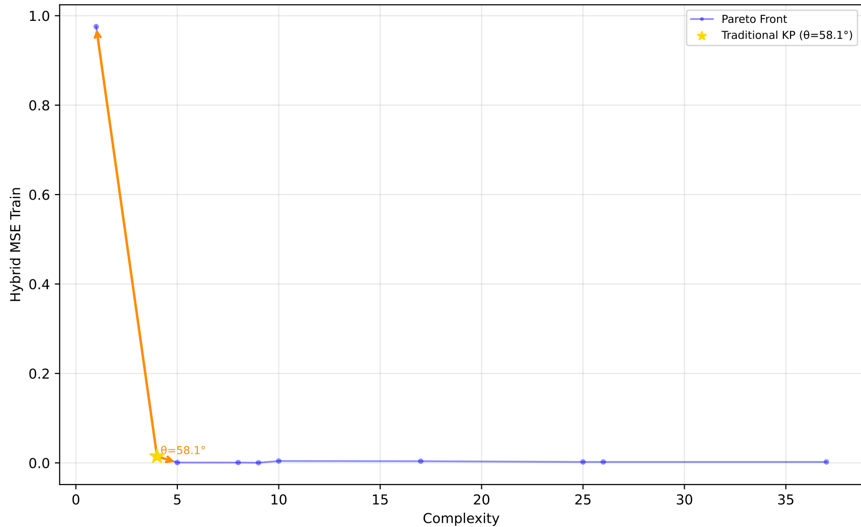
523_analcatdata_neavote - Run 20 - SVP - Hybrid MSE Train \lambda_1=0.00, \lambda_2=0.20, \lambda_3=0.00 | Difficulty: 1.00 | Method: hmr
