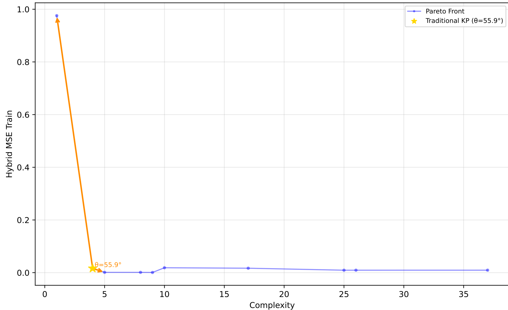
523_analcatdata_neavote - Run 20 - SVP - Hybrid MSE Train \lambda_1=0.00, \lambda_2=0.90, \lambda_3=0.00 | Difficulty: 1.00 | Method: hmr
