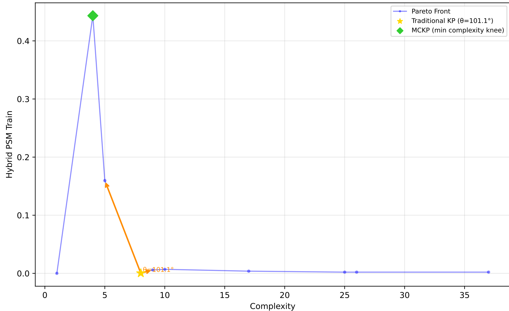
523_analcatdata_neavote - Run 20 - SVP - Hybrid PSM Train \lambda_1=0.00, \lambda_2=0.20, \lambda_3=0.00 | Difficulty: 1.00 | Method: hmr
