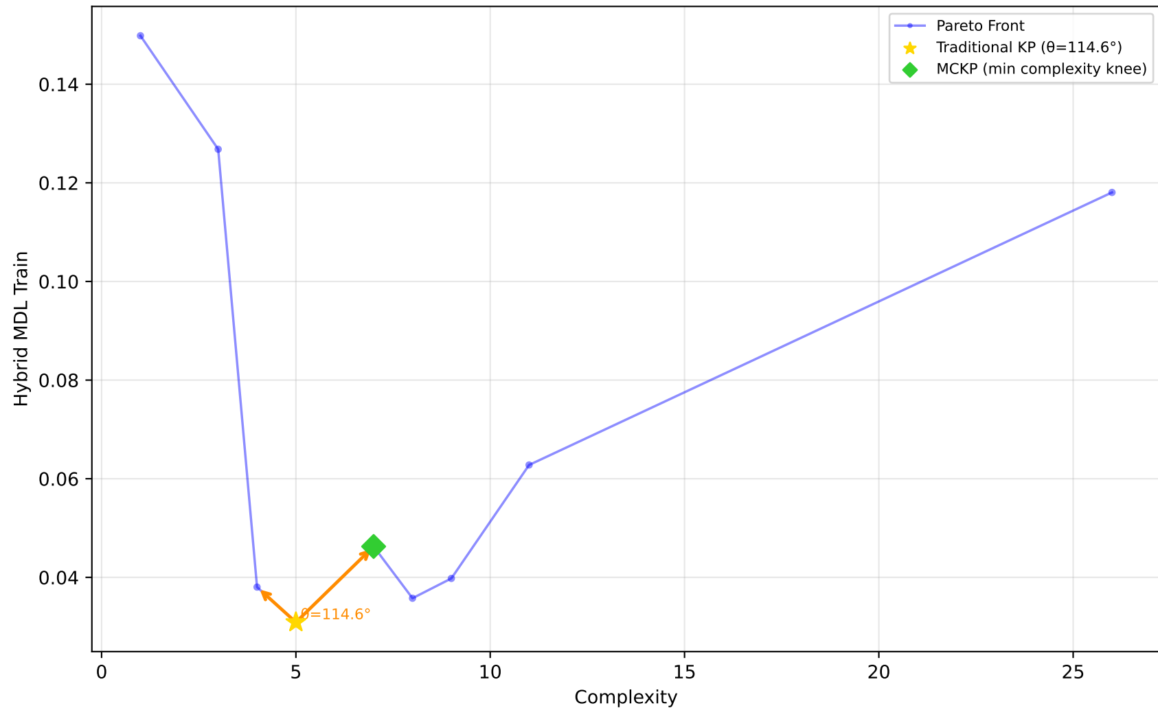
523_analcatdata_neavote - Run 21 - MVP - Hybrid MDL Train \lambda_1=0.00, \lambda_2=0.40, \lambda_3=0.00 | Difficulty: 1.00 | Method: hmr
