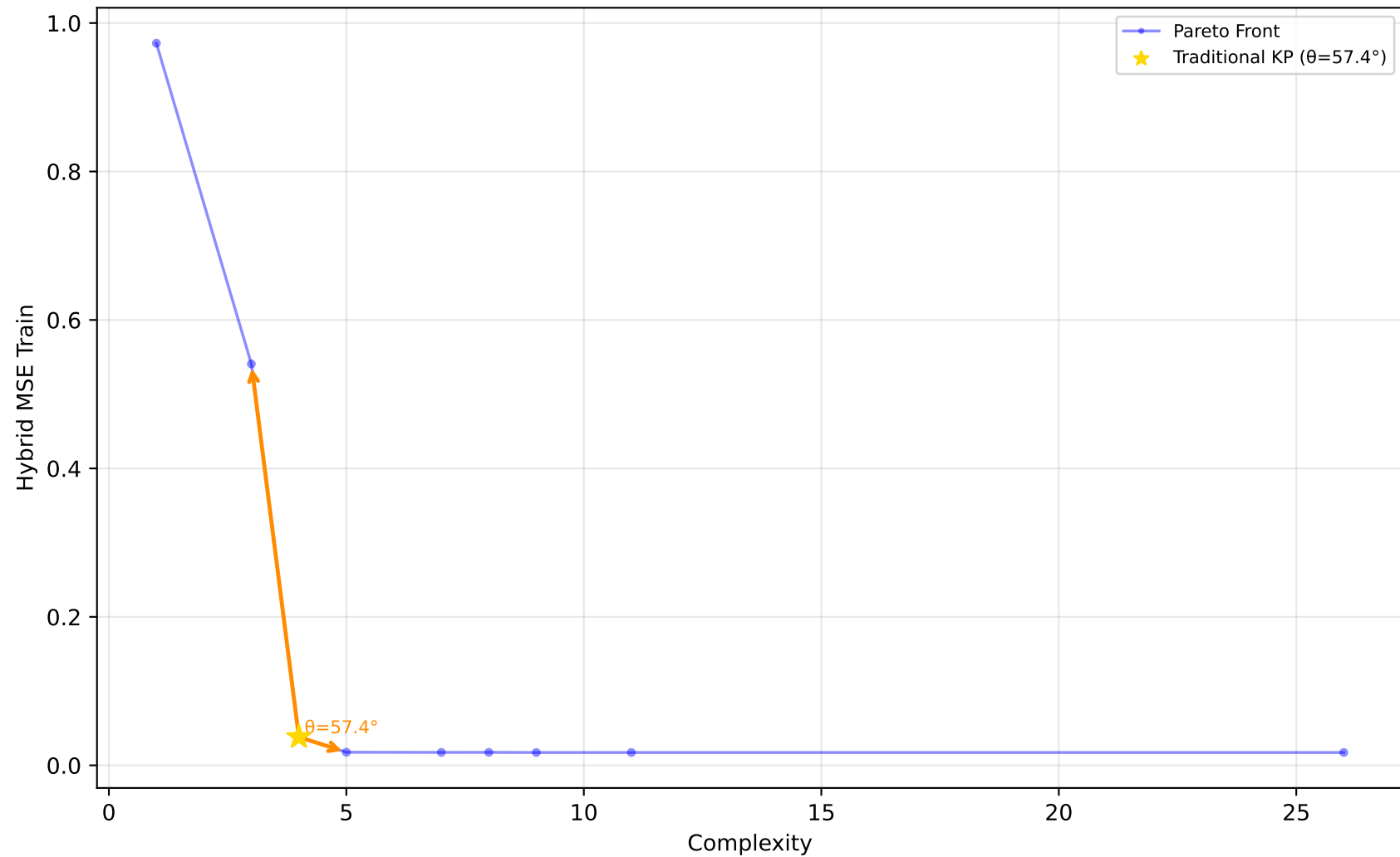
523_analcatdata_neavote - Run 21 - MVP - Hybrid MSE Train \lambda_1=0.00, \lambda_2=0.10, \lambda_3=0.00 | Difficulty: 1.00 | Method: hmr
