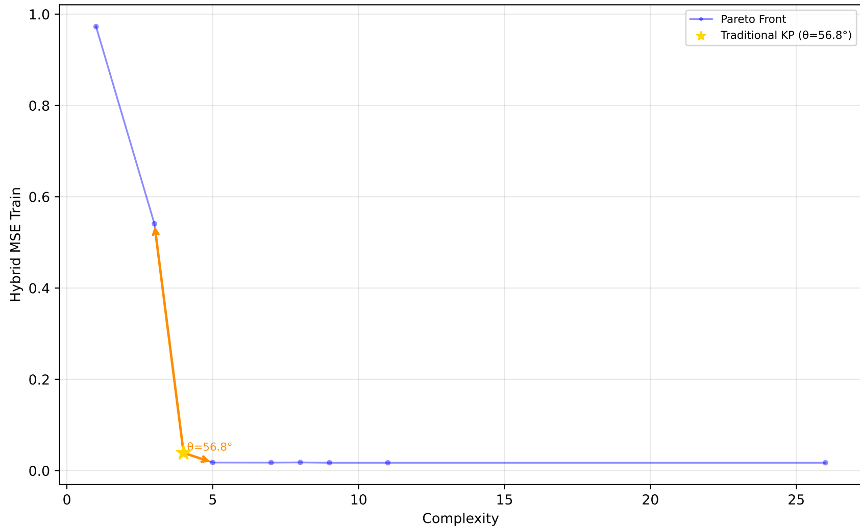
523_analcatdata_neavote - Run 21 - MVP - Hybrid MSE Train \lambda_1=0.00, \lambda_2=0.40, \lambda_3=0.00 | Difficulty: 1.00 | Method: hmr
