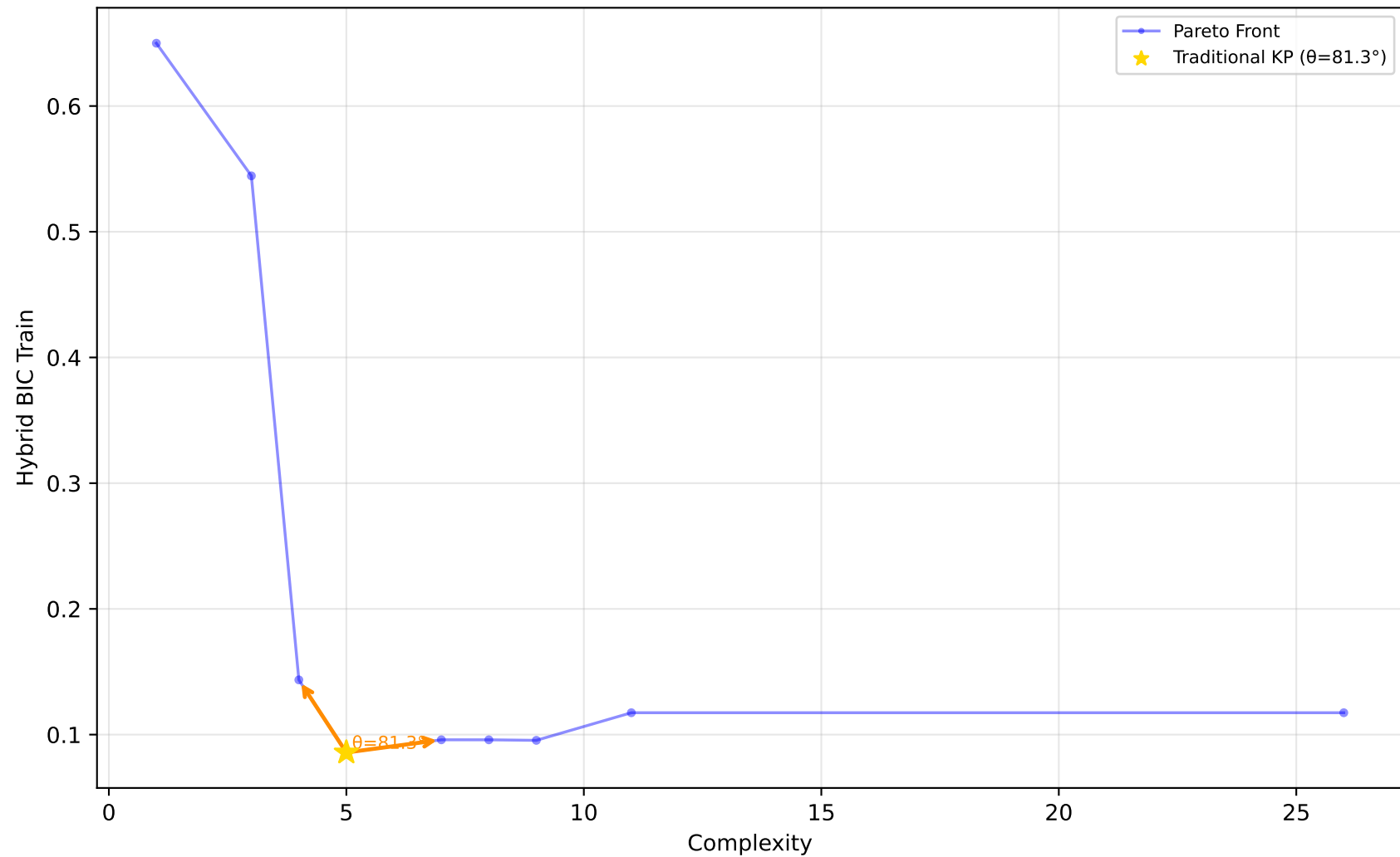
523_analcatdata_neavote - Run 21 - SVP - Hybrid BIC Train \lambda_1=0.00 , \lambda_2=0.20 , \lambda_3=0.00 | Difficulty: 1.00 | Method: hmr
