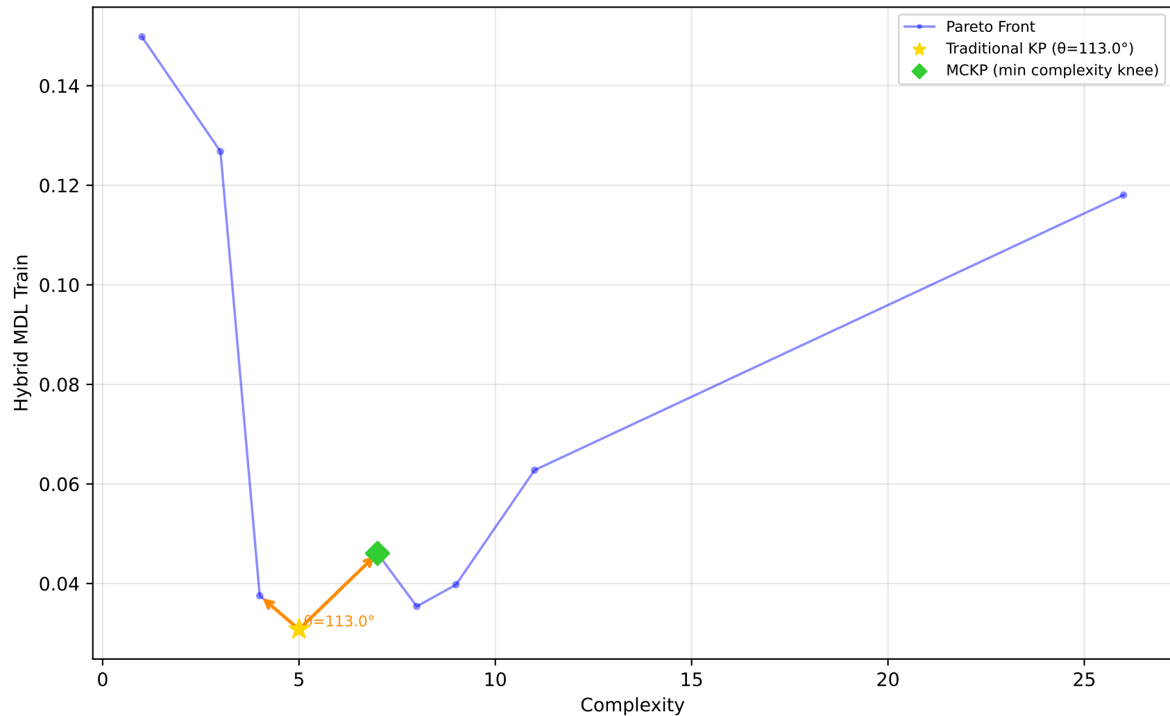
523_analcatdata_neavote - Run 21 - SVP - Hybrid MDL Train \lambda_1=0.00 , \lambda_2=0.20 , \lambda_3=0.00 | Difficulty: 1.00 | Method: hmr
