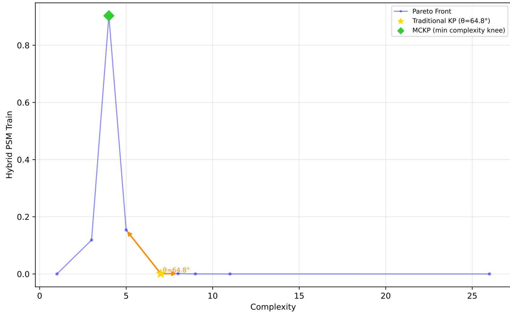
523_analcatdata_neavote - Run 21 - SVP - Hybrid PSM Train \lambda_1=0.00 , \lambda_2=0.20 , \lambda_3=0.00 | Difficulty: 1.00 | Method: hmr
