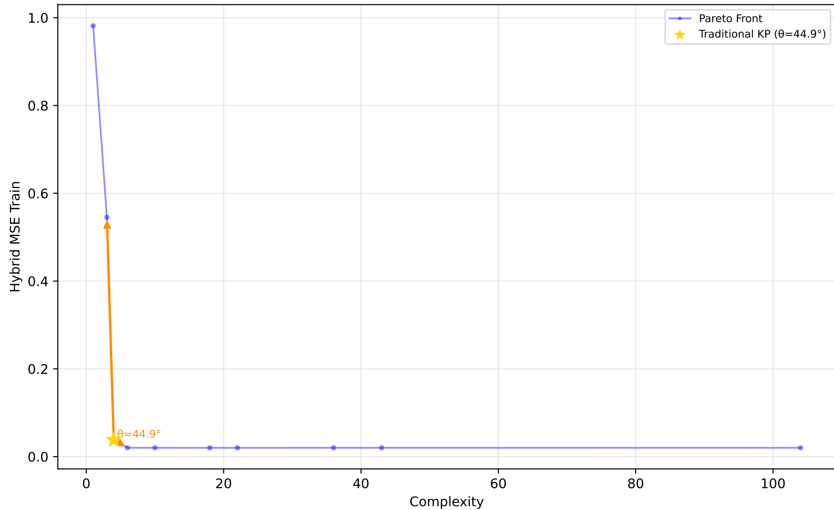
523_analcatdata_neavote - Run 22 - MVP - Hybrid MSE Train \lambda_1=0.00, \lambda_2=0.10, \lambda_3=0.00 | Difficulty: 1.00 | Method: hmr
