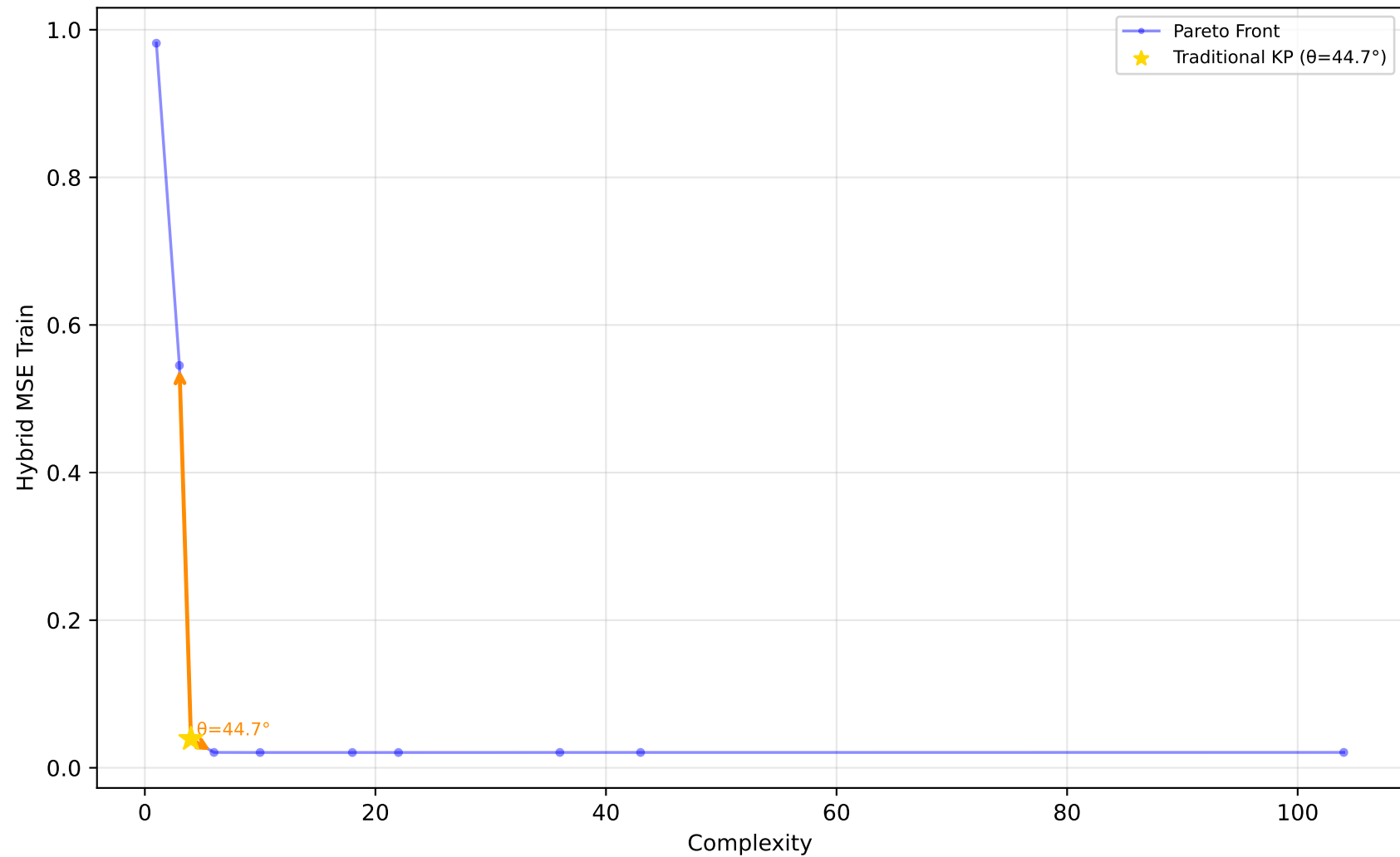
523_analcatdata_neavote - Run 22 - MVP - Hybrid MSE Train \lambda_1=0.00, \lambda_2=0.40, \lambda_3=0.00 | Difficulty: 1.00 | Method: hmr
