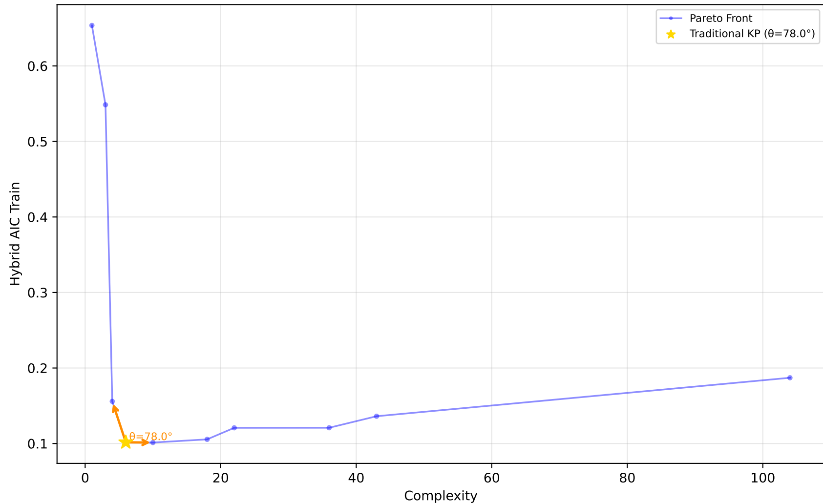
523_analcatdata_neavote - Run 22 - SVP - Hybrid AIC Train \lambda_1=0.00, \lambda_2=0.90, \lambda_3=0.00 | Difficulty: 1.00 | Method: hmr
