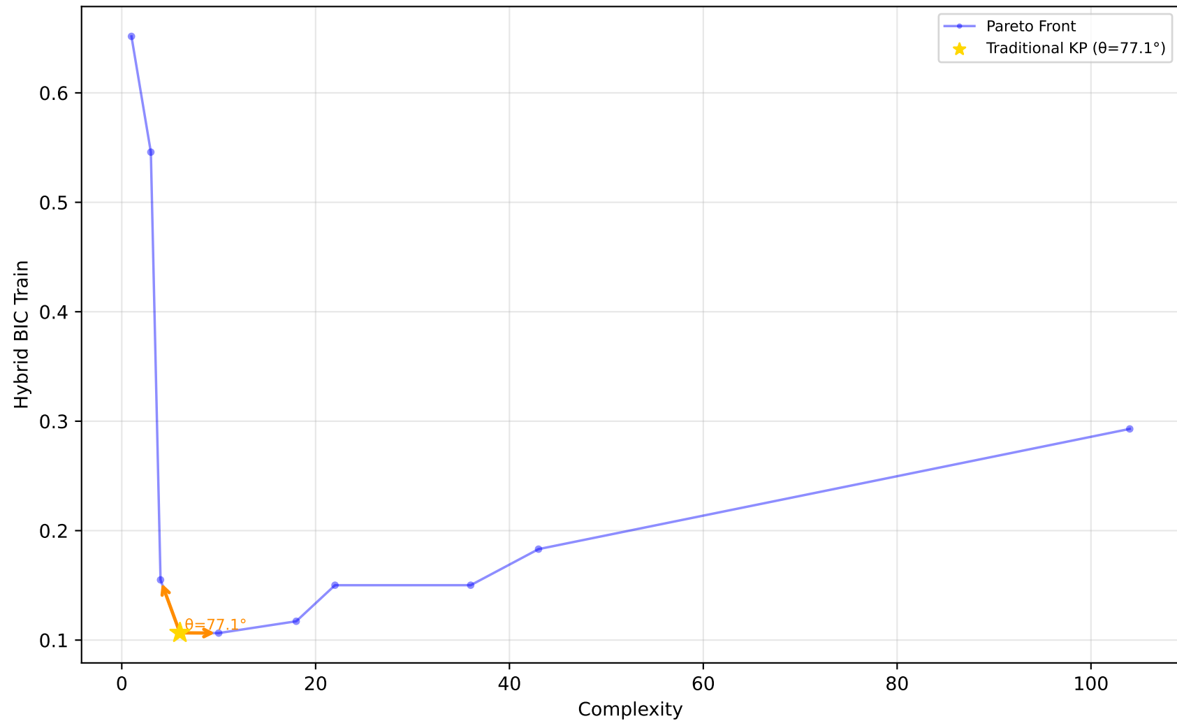
523_analcatdata_neavote - Run 22 - SVP - Hybrid BIC Train \lambda_1=0.00 , \lambda_2=0.20 , \lambda_3=0.00 | Difficulty: 1.00 | Method: hmr
