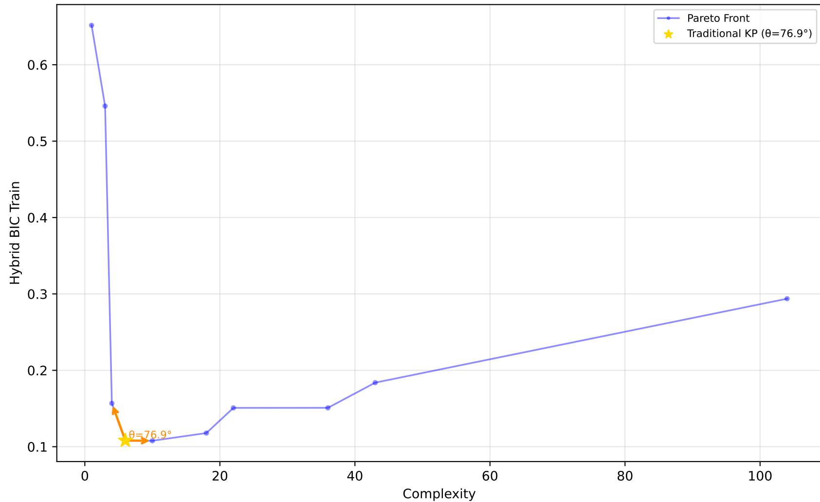
523_analcatdata_neavote - Run 22 - SVP - Hybrid BIC Train \lambda_1=0.00, \lambda_2=0.90, \lambda_3=0.00 | Difficulty: 1.00 | Method: hmr
