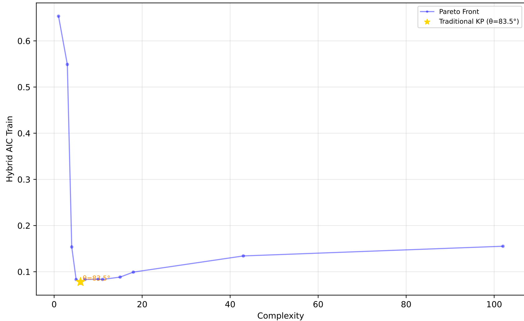
523_analcatdata_neavote - Run 23 - MVP - Hybrid AIC Train \lambda_1=0.00 , \lambda_2=0.10 , \lambda_3=0.00 | Difficulty: 1.00 | Method: hmr
