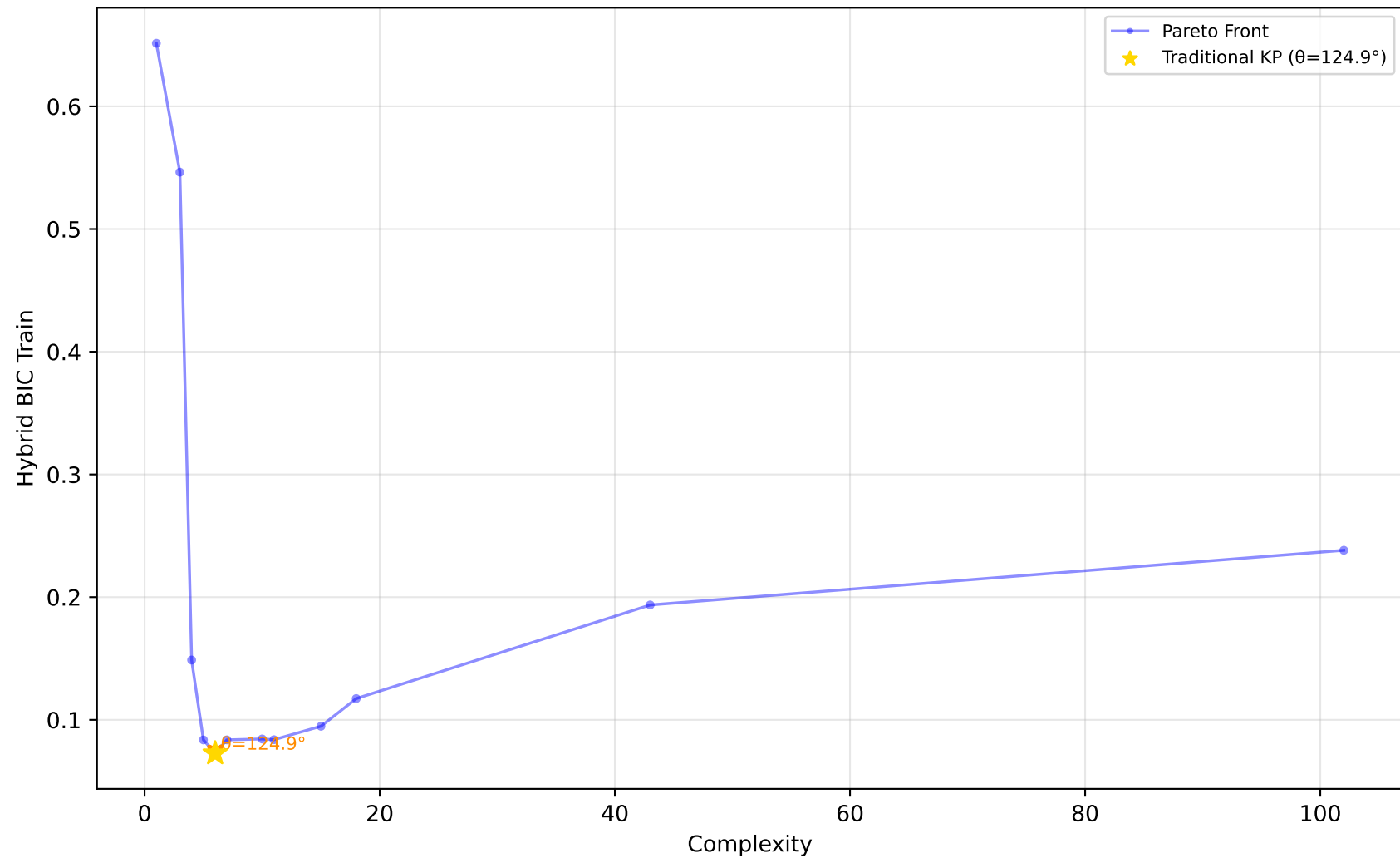
523_analcatdata_neavote - Run 23 - MVP - Hybrid BIC Train \lambda_1=0.00, \lambda_2=0.10, \lambda_3=0.00 | Difficulty: 1.00 | Method: hmr
