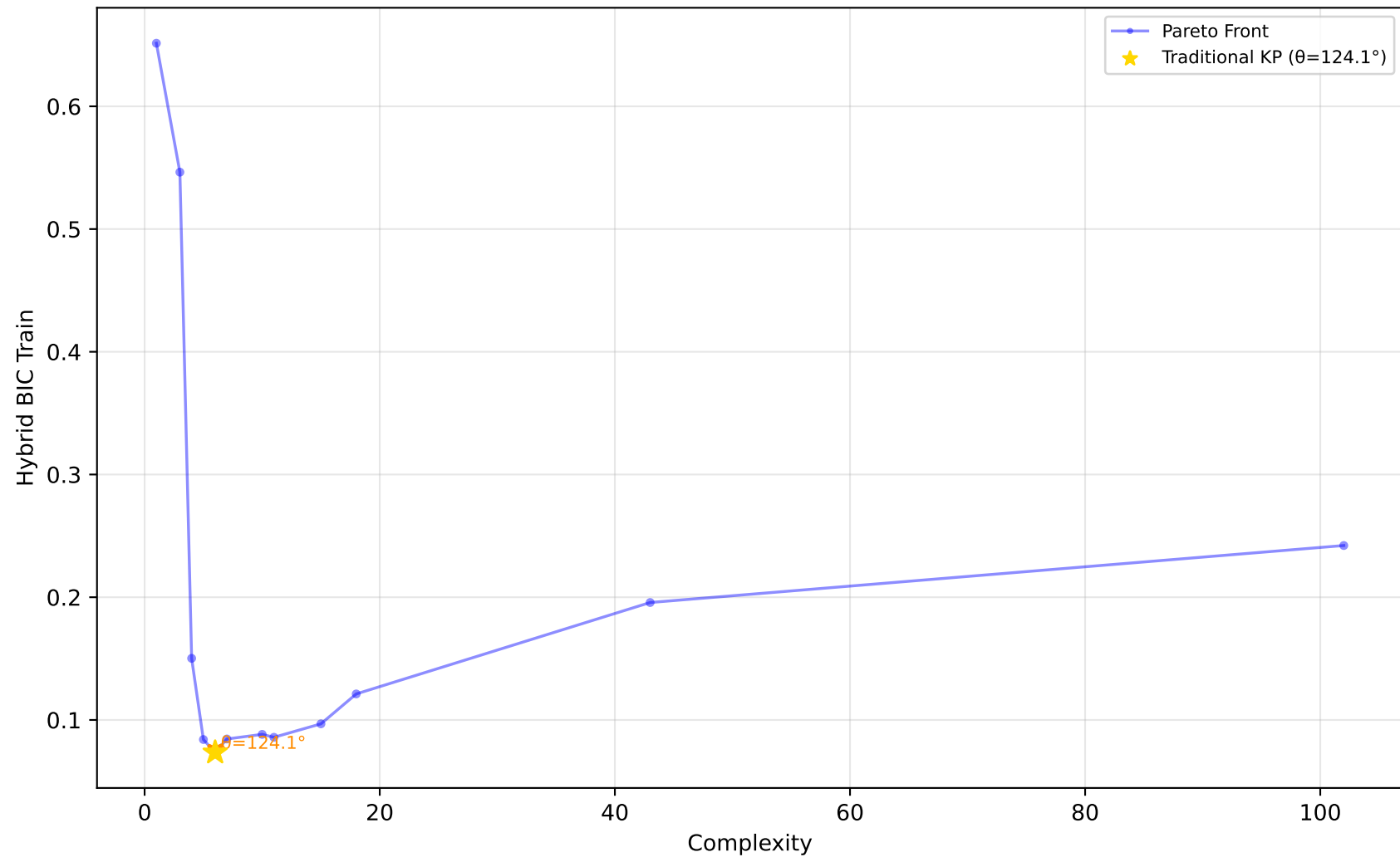
523_analcatdata_neavote - Run 23 - MVP - Hybrid BIC Train \lambda_1=0.00 , \lambda_2=0.40 , \lambda_3=0.00 | Difficulty: 1.00 | Method: hmr
