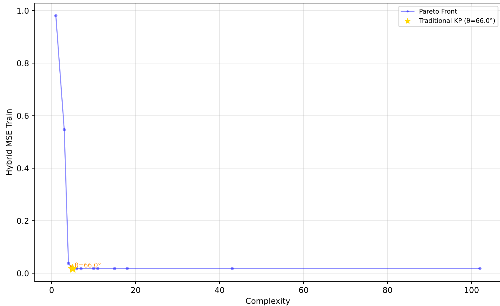
523_analcatdata_neavote - Run 23 - MVP - Hybrid MSE Train \lambda_1=0.00, \lambda_2=0.10, \lambda_3=0.00 | Difficulty: 1.00 | Method: hmr
