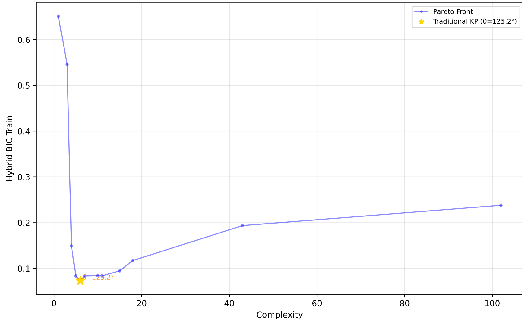
523_analcatdata_neavote - Run 23 - SVP - Hybrid BIC Train \lambda_1=0.00 , \lambda_2=0.20 , \lambda_3=0.00 | Difficulty: 1.00 | Method: hmr
