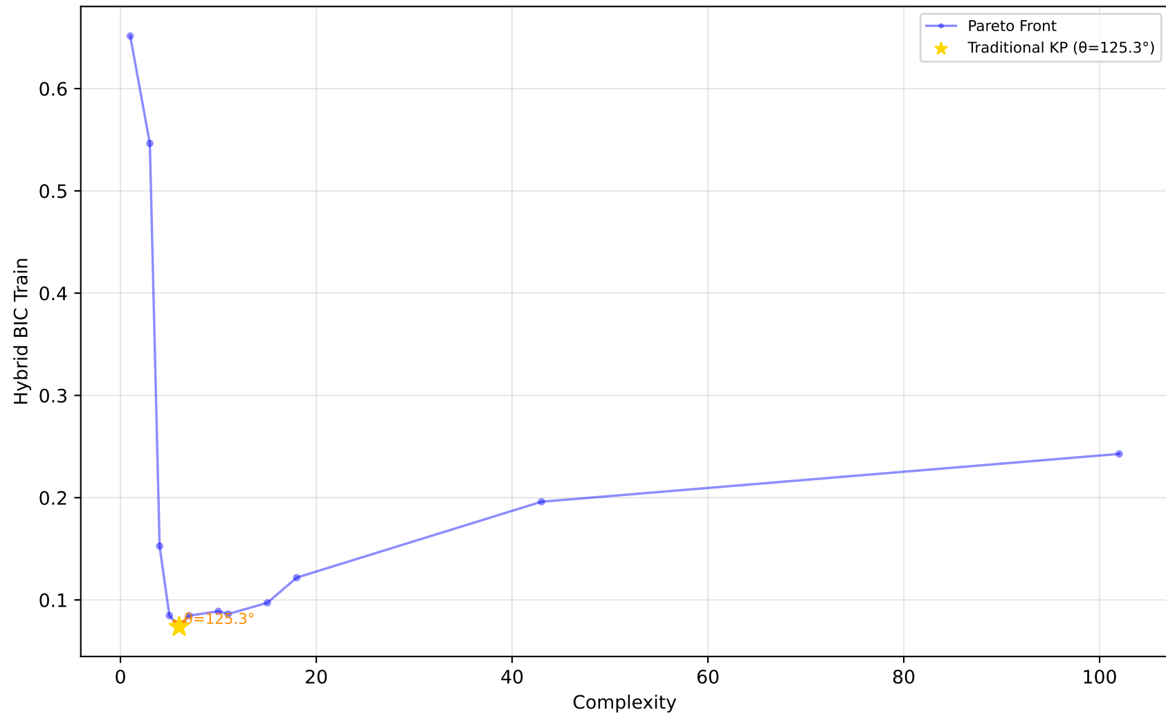
523_analcatdata_neavote - Run 23 - SVP - Hybrid BIC Train \lambda_1=0.00, \lambda_2=0.90, \lambda_3=0.00 | Difficulty: 1.00 | Method: hmr
