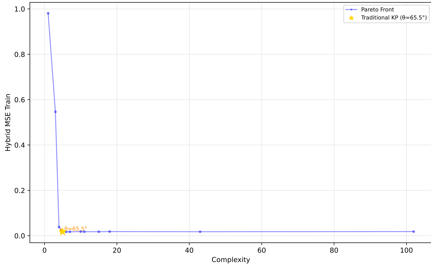
523_analcatdata_neavote - Run 23 - SVP - Hybrid MSE Train \lambda_1=0.00, \lambda_2=0.20, \lambda_3=0.00 | Difficulty: 1.00 | Method: hmr
