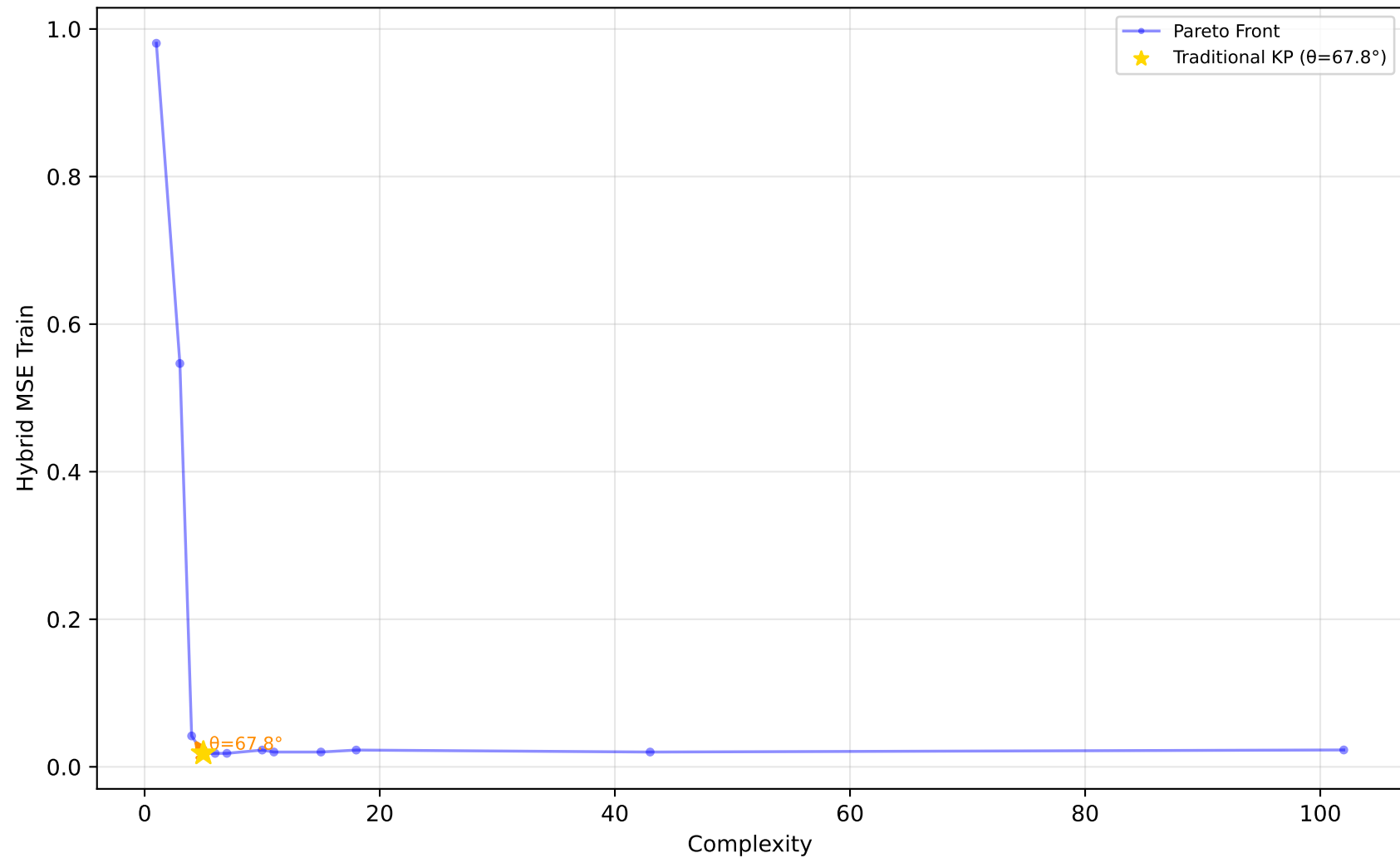
523_analcatdata_neavote - Run 23 - SVP - Hybrid MSE Train \lambda_1=0.00, \lambda_2=0.90, \lambda_3=0.00 | Difficulty: 1.00 | Method: hmr
