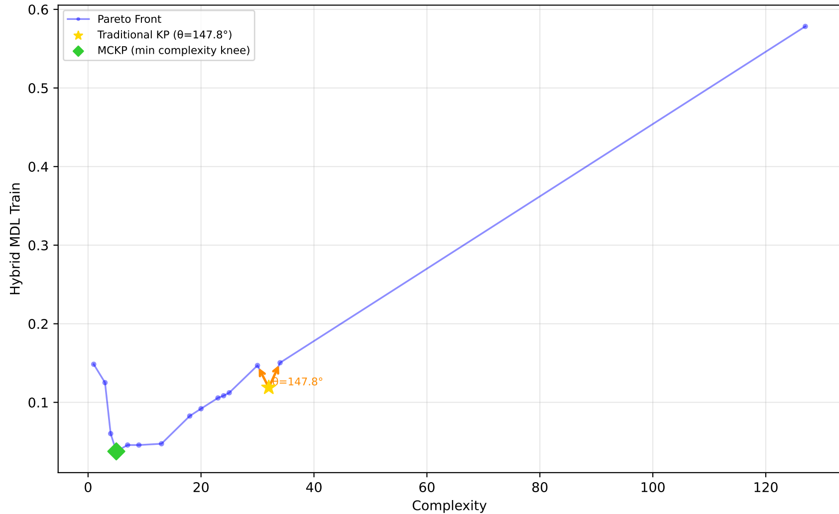
523_analcatdata_neavote - Run 24 - MVP - Hybrid MDL Train \lambda_1=0.00, \lambda_2=0.10, \lambda_3=0.00 | Difficulty: 1.00 | Method: hmr
